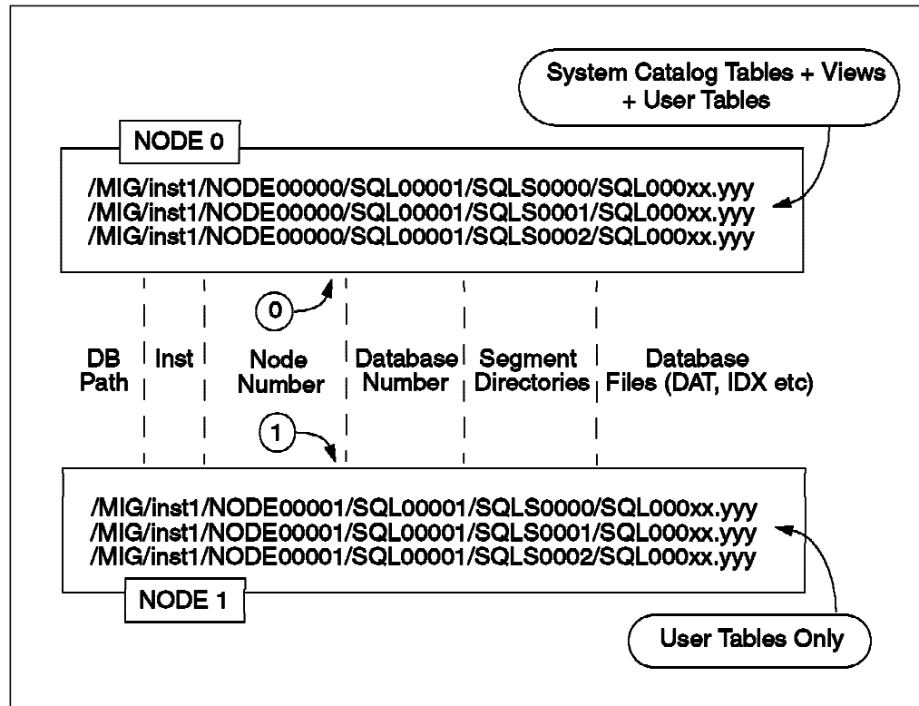
Figure 182. Physical View before Migration
