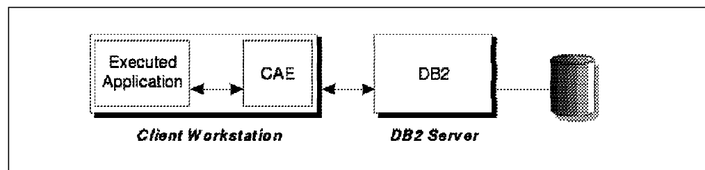
Figure 3. Remote Client Accessing DB2 Server Using CAE
