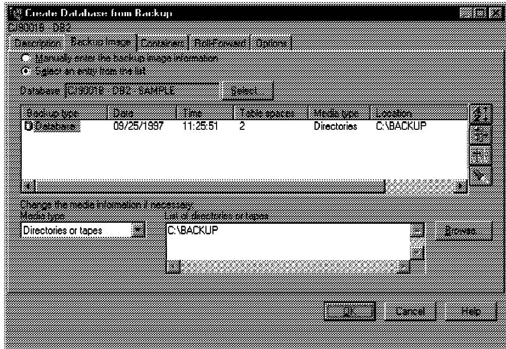
Figure 75. Creating a Database from Backup Image
