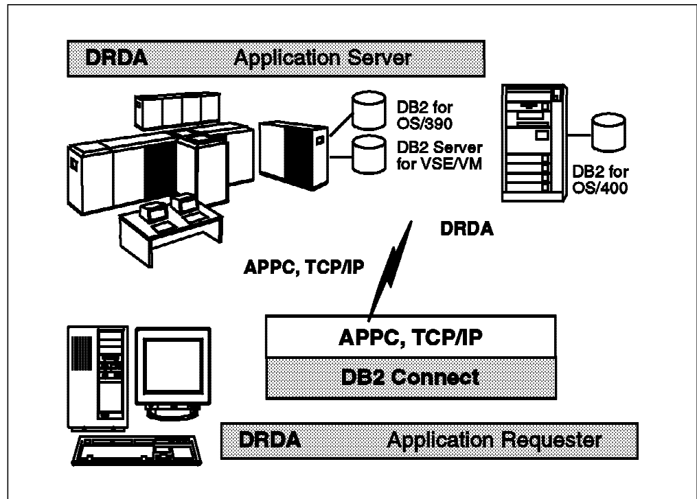
Figure 8. DRDA Application Flow
