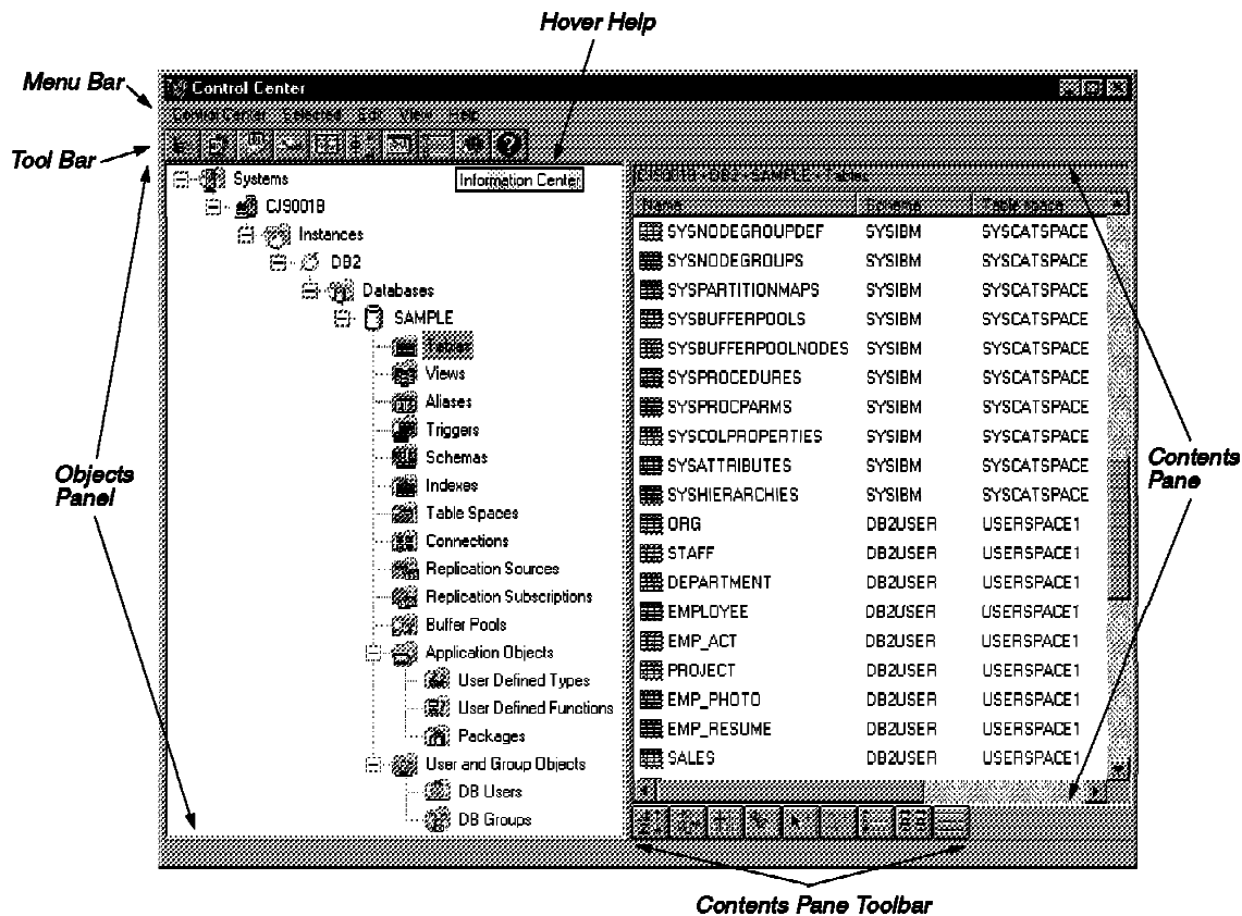
Figure 67. Main Components of the Control Center
