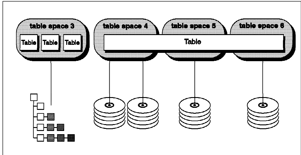
Figure 50. Table Spaces and Containers
