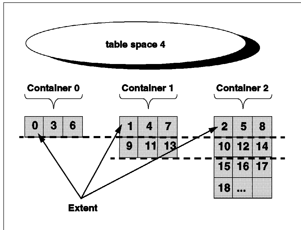
Figure 55. Writing to Containers
