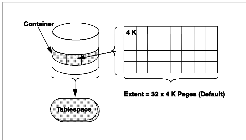
Figure 52. Extents, Containers and Table Spaces
