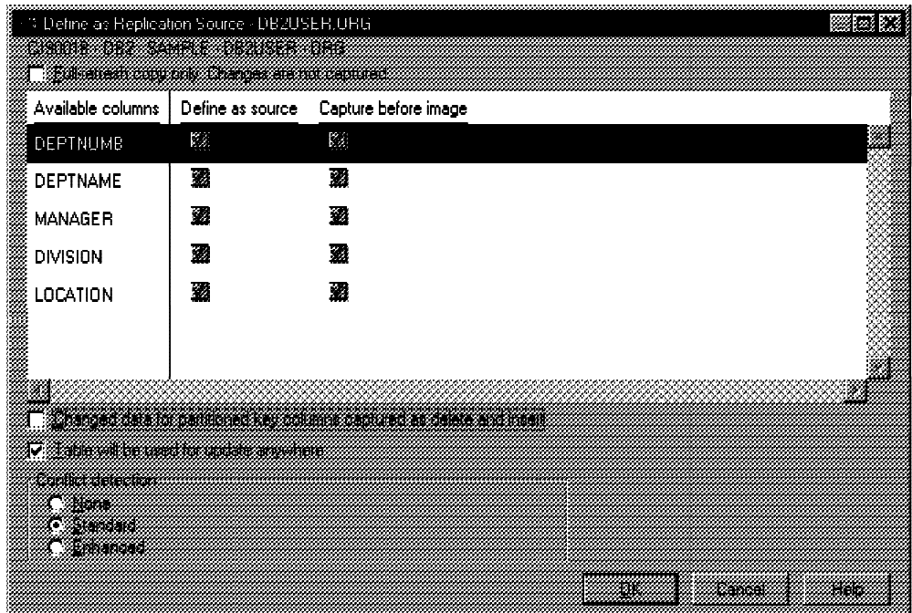
Figure 86. Defining a Replication Source
