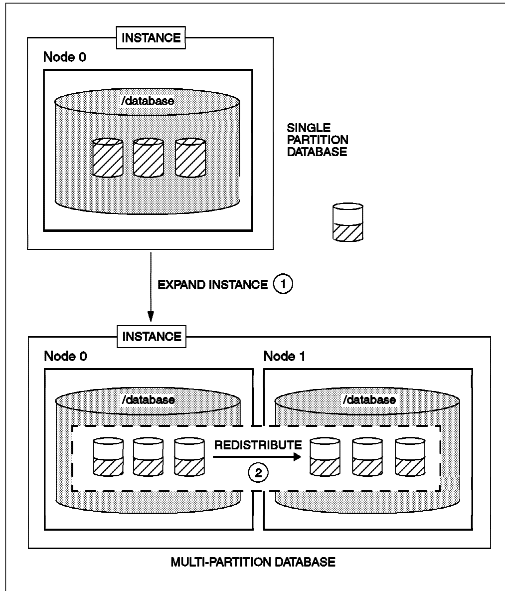
Figure 177. The Redistribute Method
