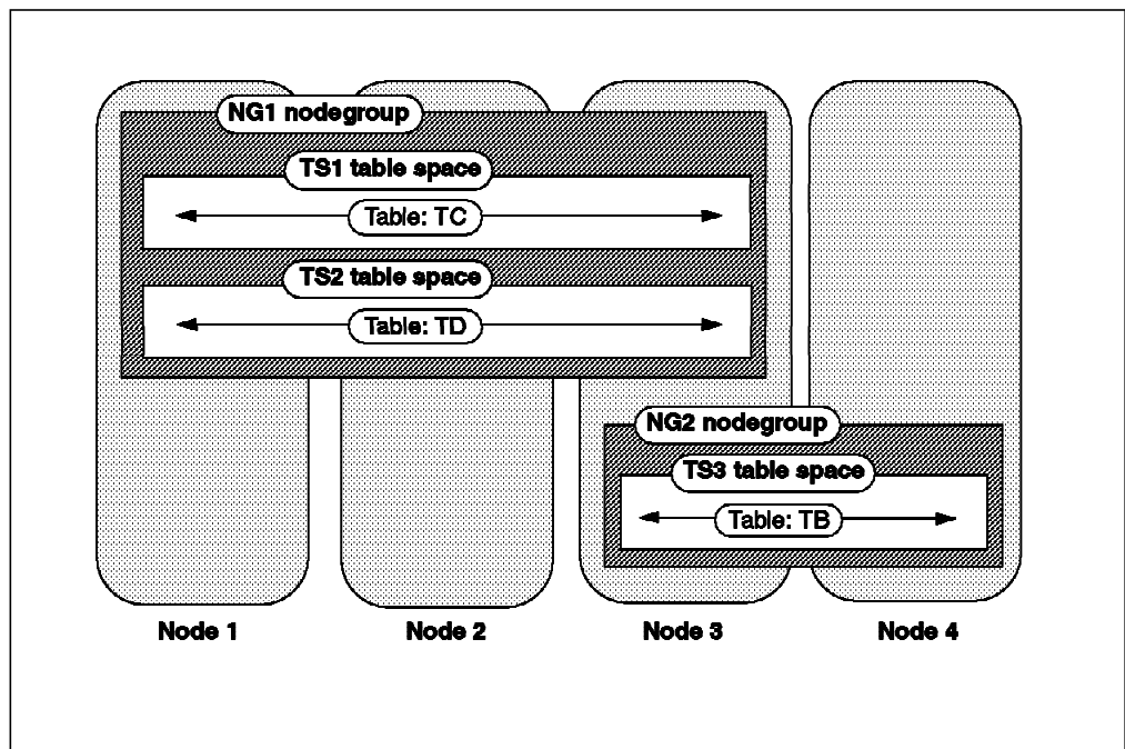
Figure 51. Nodegroups, Table Spaces and Tables
