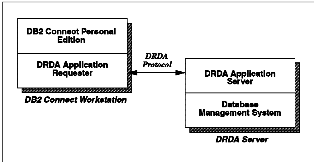
Figure 9. DRDA Flow in DB2 Connect Personal Edition
