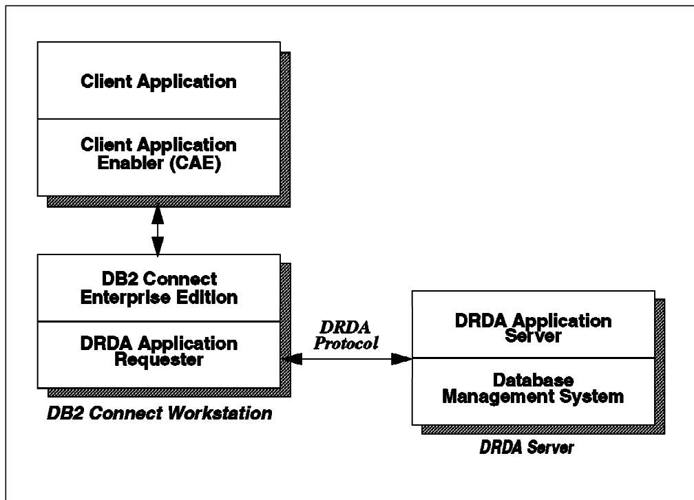
Figure 10. DRDA Flow in DB2 Connect Enterprise Edition
