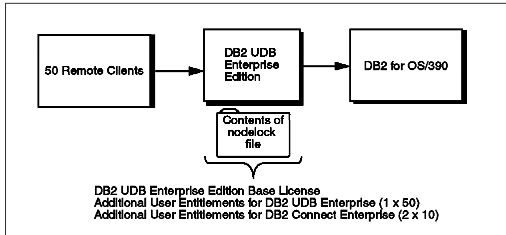
Figure 12. Increasing the Number of Users
