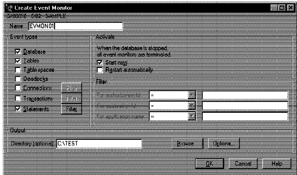
Figure 108. Creating an Event Monitor
