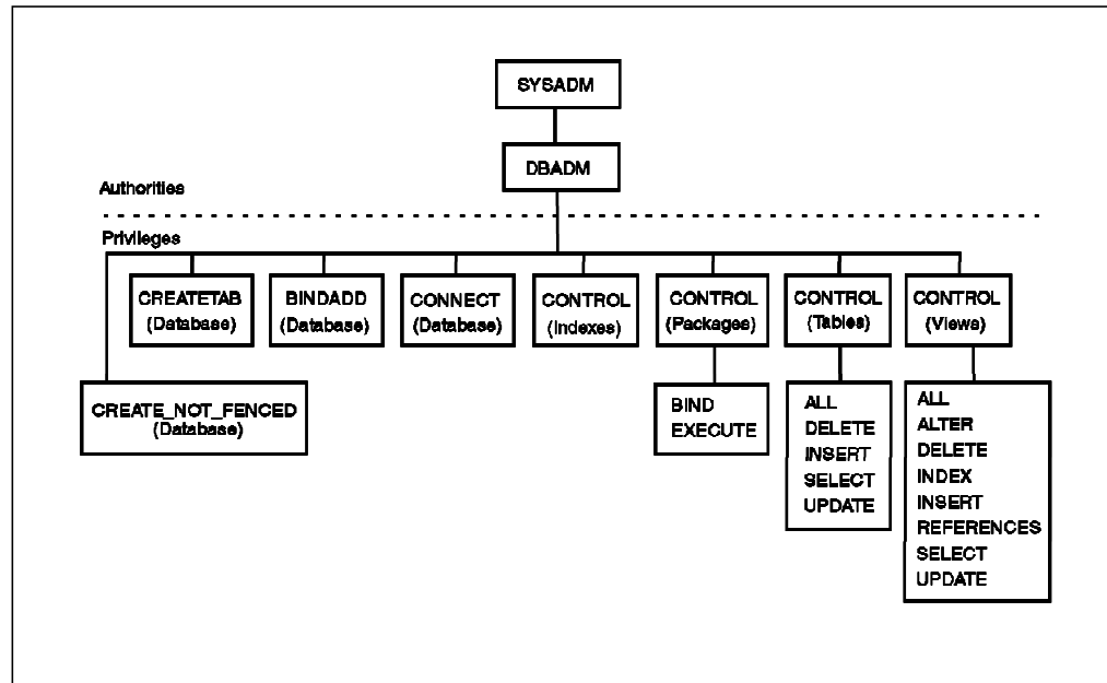
Figure 59. Authorities and Privileges
