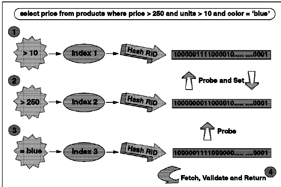
Figure 34. Dynamic Bitmap Index ANDing
