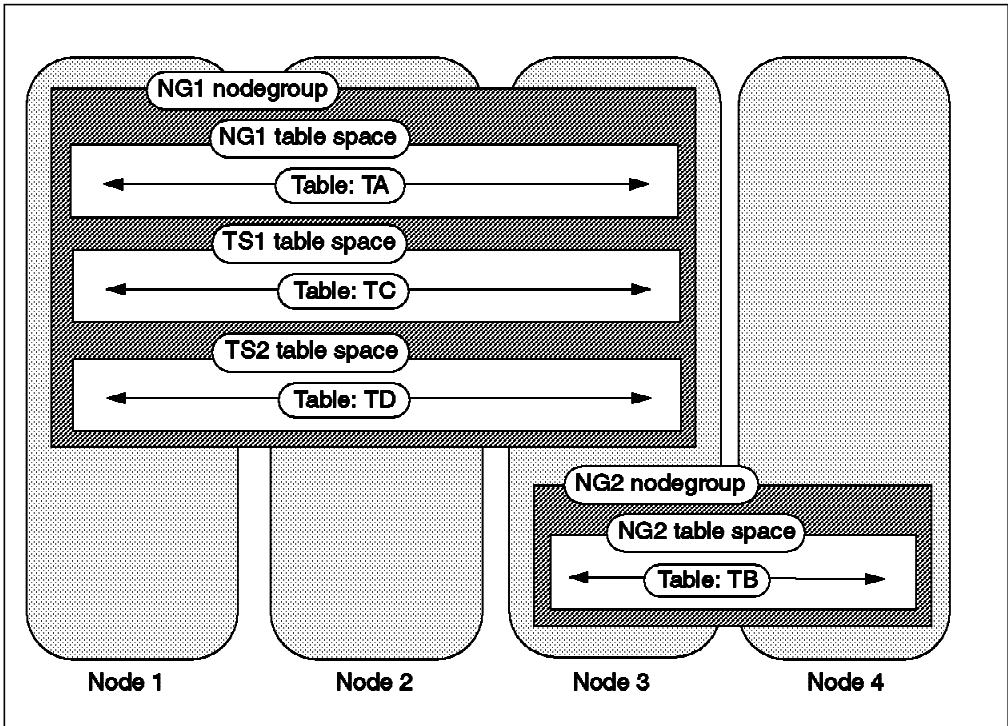
Figure 180. Customized Table Spaces Created during Database Migration
