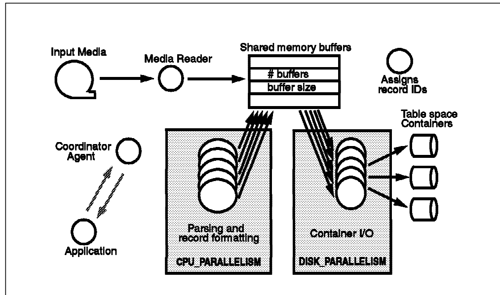
Figure 30. Load Parallelism
