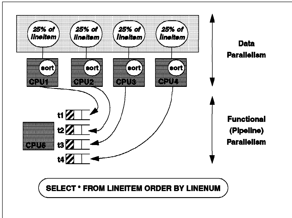
Figure 28. Data and Functional Parallelism
