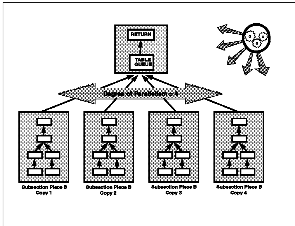
Figure 27. Degree of Parallelism
