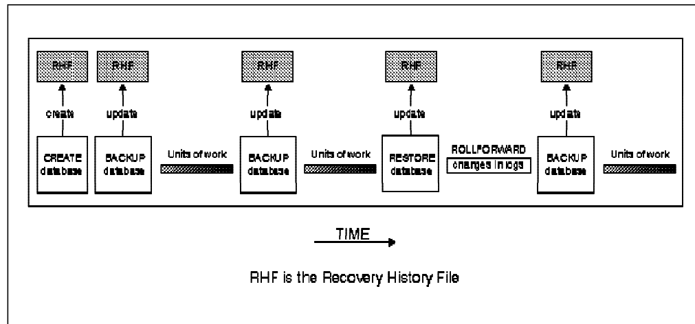
Figure 56. Creating and Updating the Recovery History File
