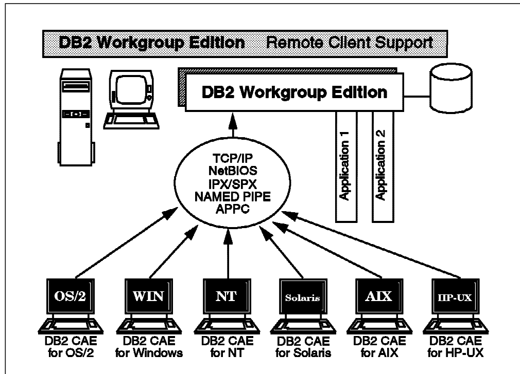
Figure 5. DB2 Workgroup Edition with Remote Clients
