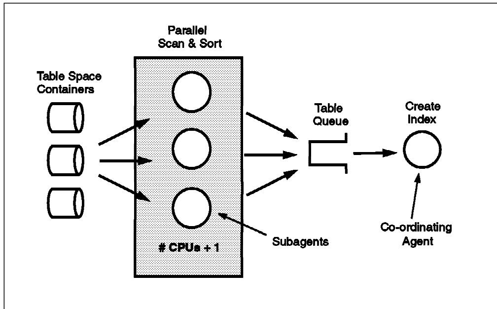
Figure 31. Index Create Parallelism
