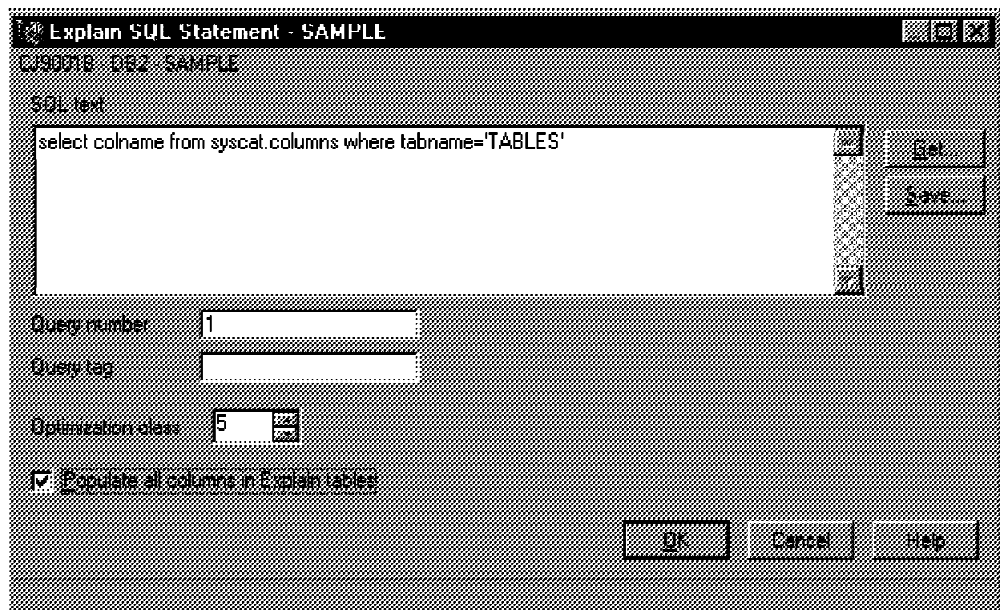
Figure 101. Explaining an SQL Statement
