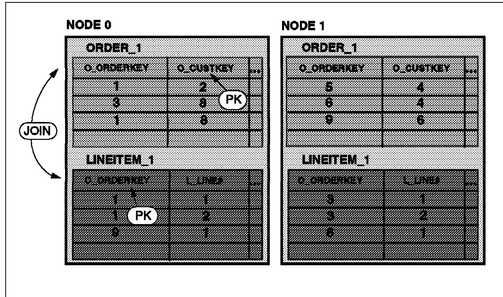
Figure 44. Directed Inner Join
