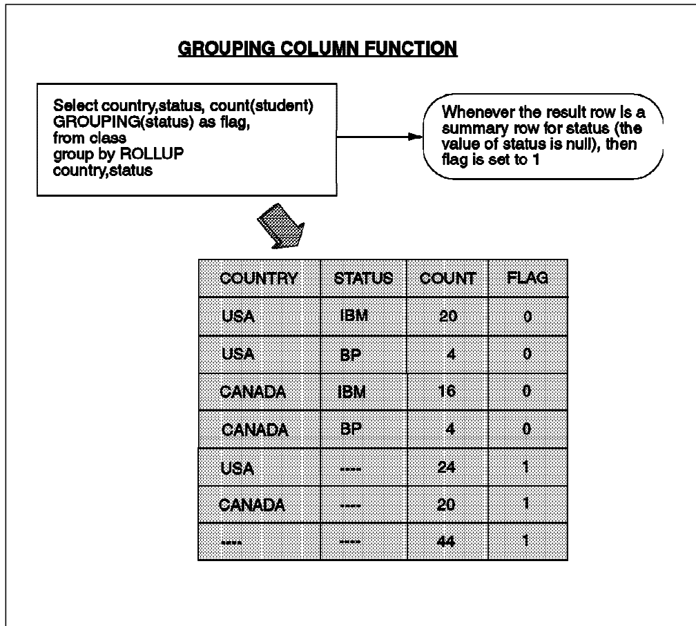
Figure 42. Example of the Grouping Column Function
