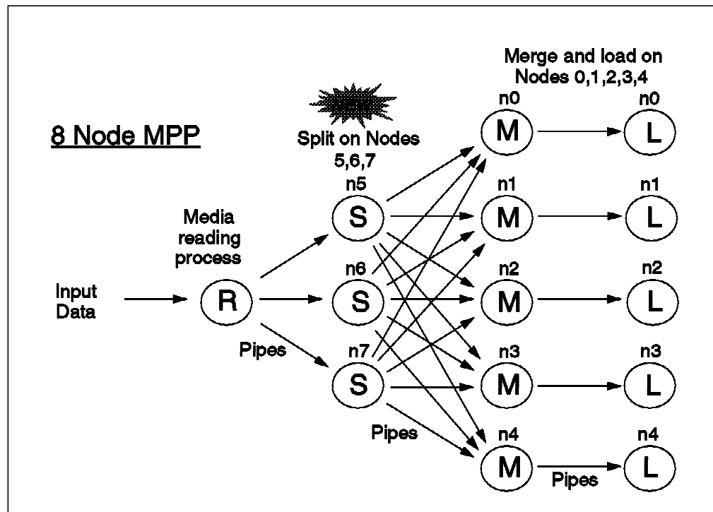
Figure 21. Multi-Node Load - db2split
