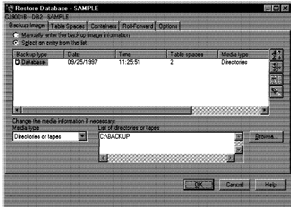
Figure 93. Restore Database Notebook
