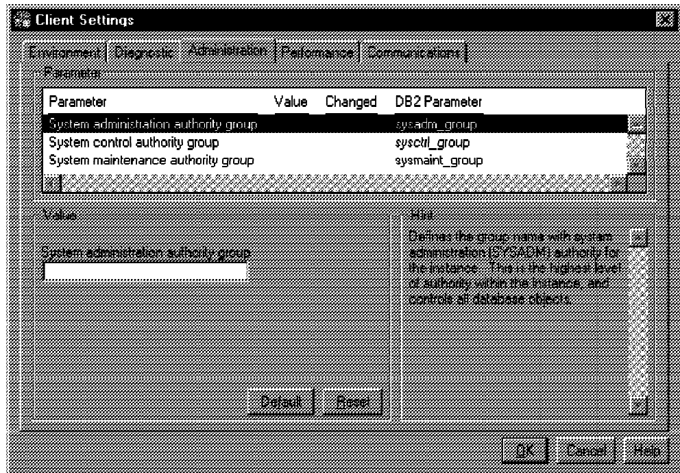
Figure 98. Updating Database Manager Configuration Parameters for Administration
