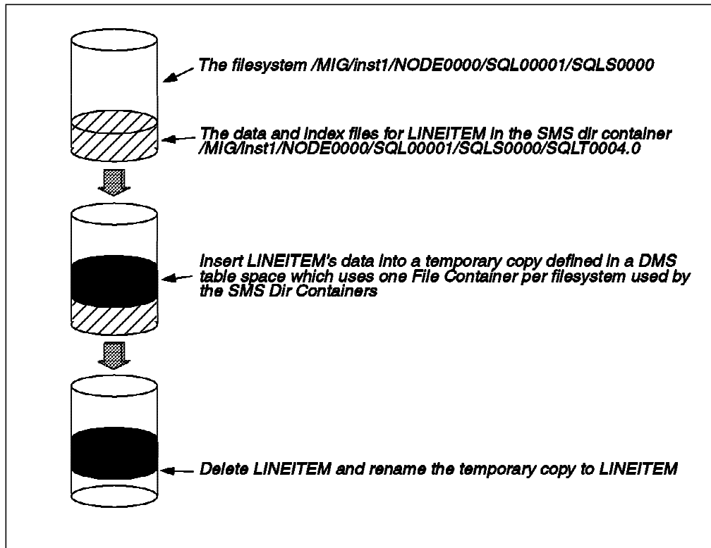
Figure 185. Insert Subselect Method
