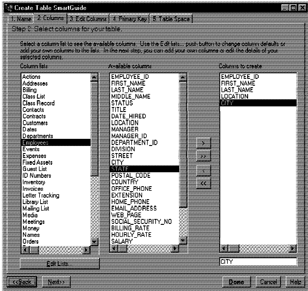
Figure 79. Create Table SmartGuide
