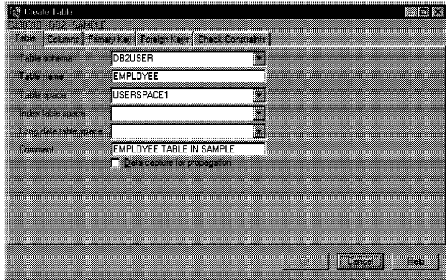
Figure 78. Create Table Notebook
