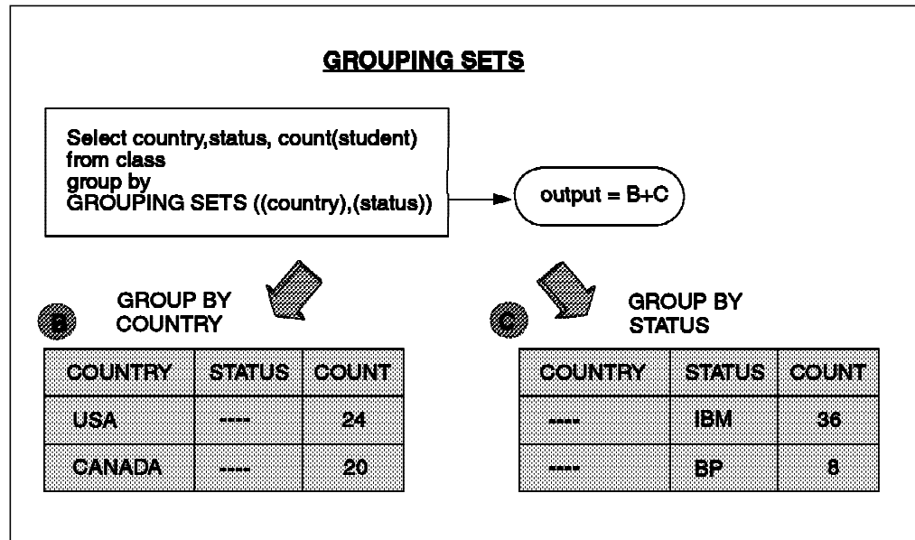
Figure 41. Example of Grouping Sets
