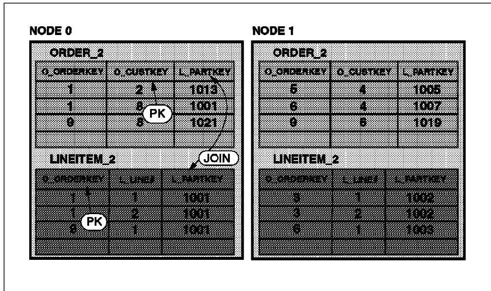
Figure 45. Broadcast Inner Join
