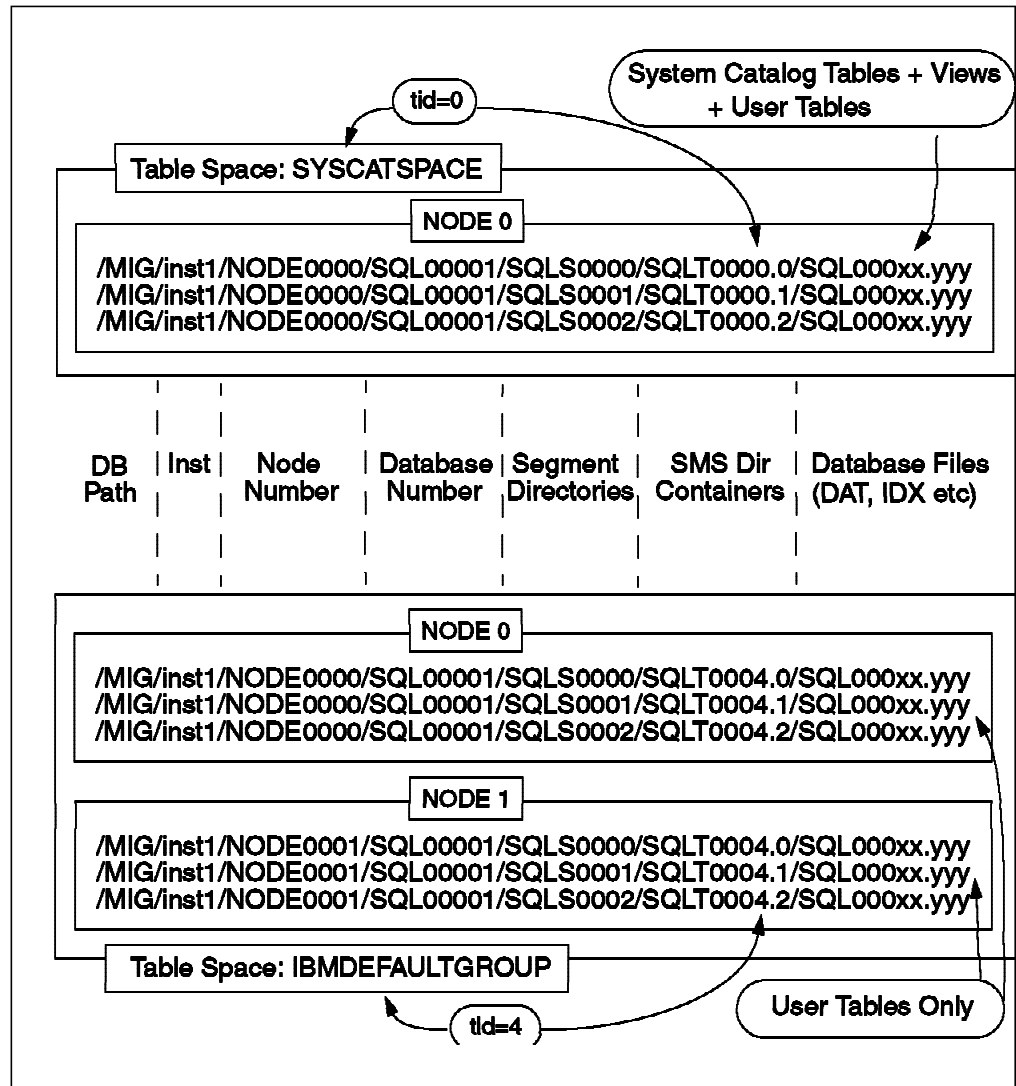
Figure 184. Physical View after Migration
