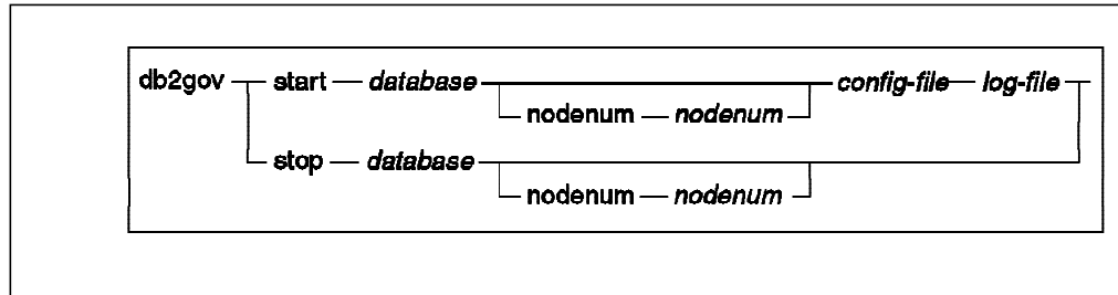
Figure 22. DB2 Governor Command Syntax
