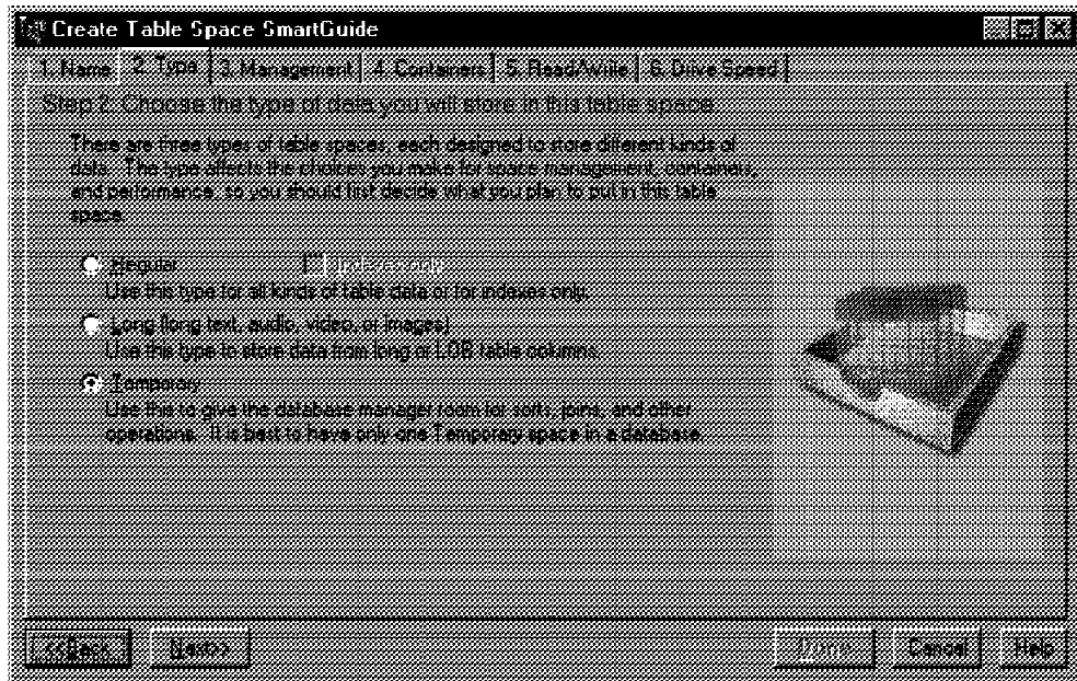
Figure 77. Create Table Space SmartGuide
