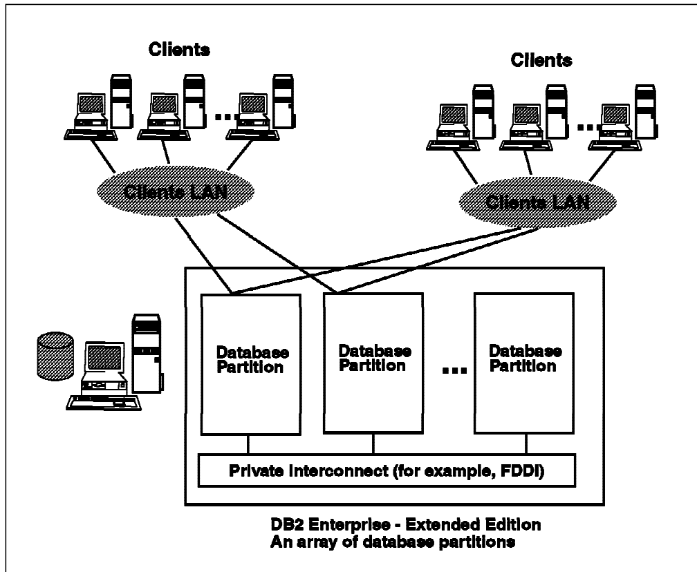
Figure 7. DB2 Enterprise - Extended Edition
