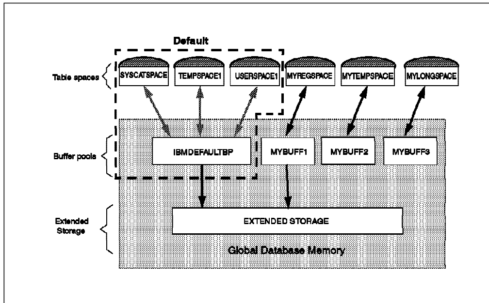
Figure 16. Buffer Pool Overview
