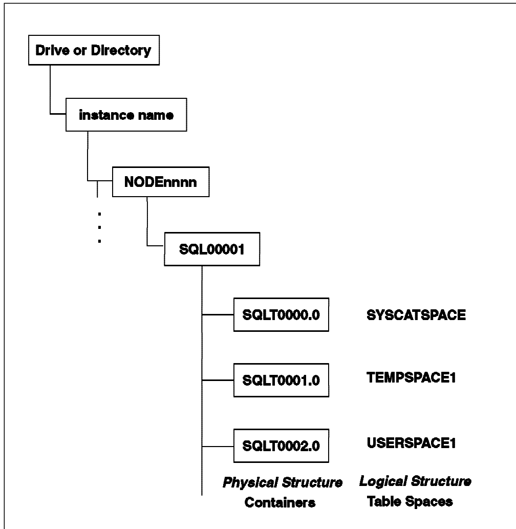
Figure 54. Table Spaces Created with Default Database Configuration
