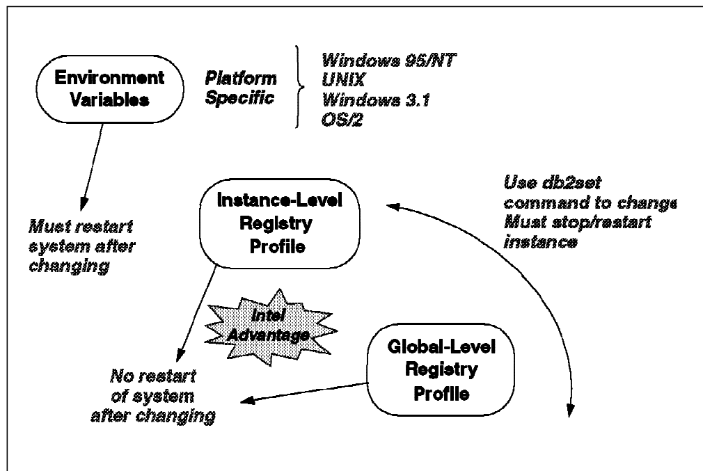
Figure 48. Environment Variables and Profile Registries
