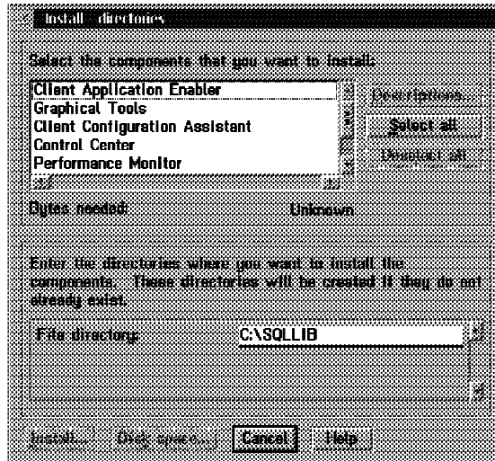
Figure 171. OS/2 DB2 UDB V5 CAE Install - directories
