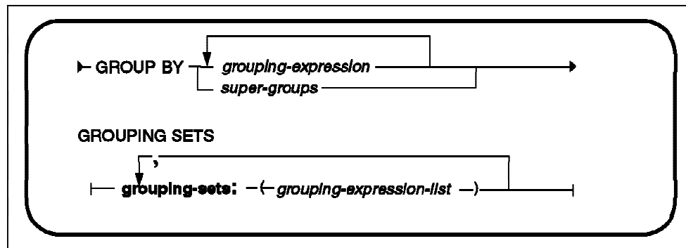
Figure 40. Grouping Sets Syntax
