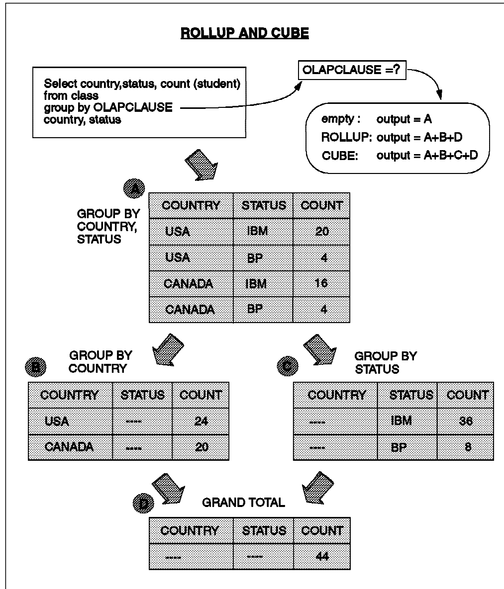
Figure 39. Example of Rollup and Cube
