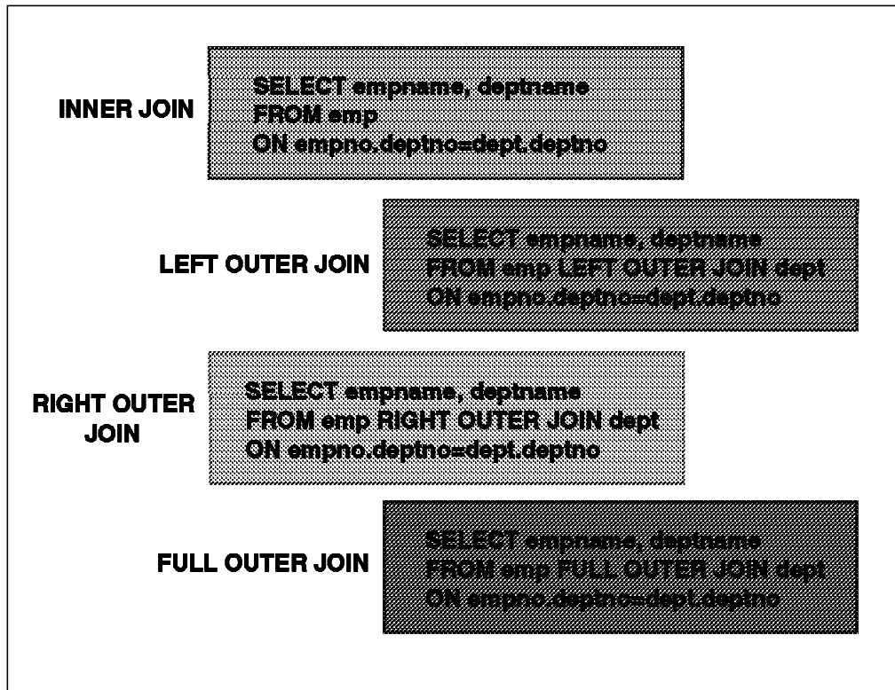
Figure 43. Inner and Outer Joins
