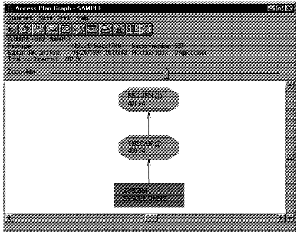
Figure 102. Graphical Representation of an SQL Statement Access Plan
