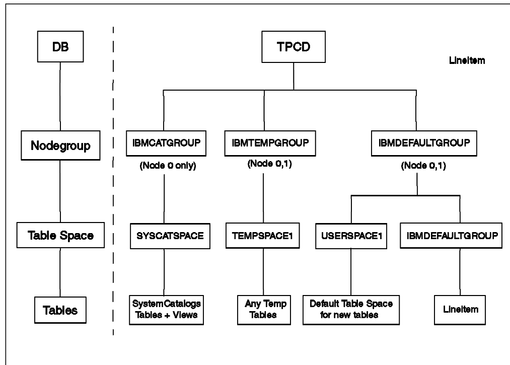
Figure 183. Logical View after Migration
