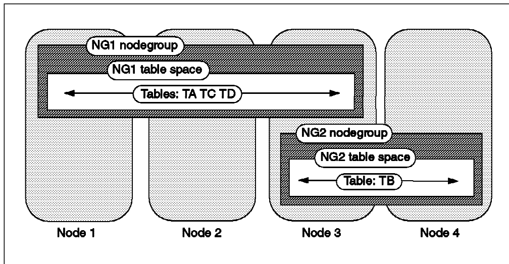
Figure 179. Default Table Spaces Created during Database Migration
