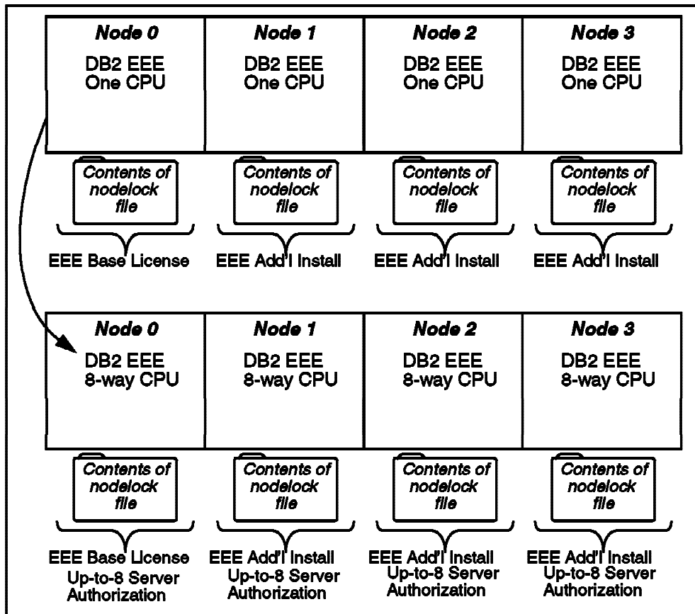
Figure 14. Increasing the Number of Processors
