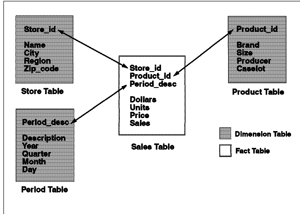
Figure 35. Star Join Visualization
