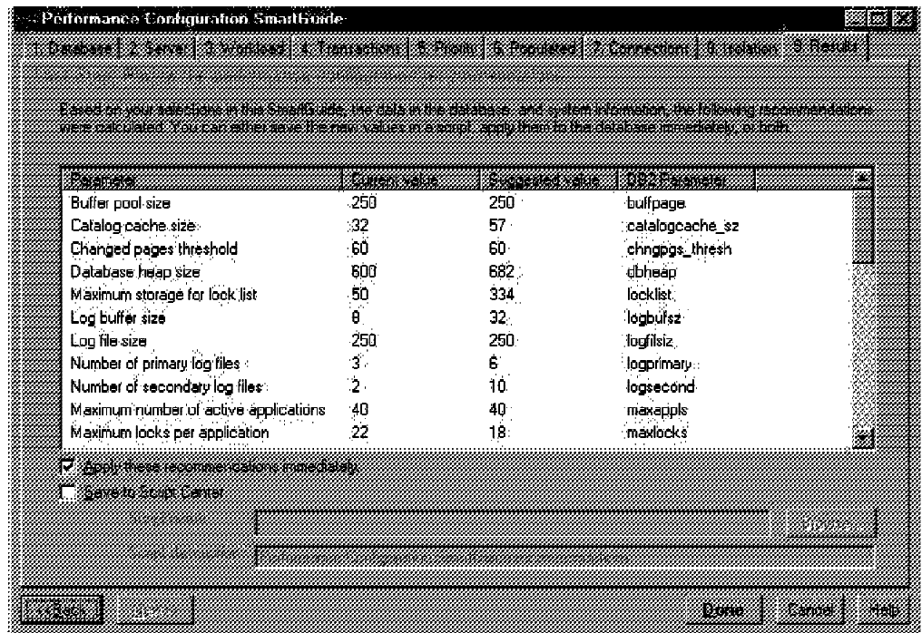
Figure 47. SmartGuide for Performance
