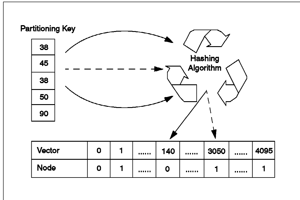
Figure 175. How db2split Partitions Data
