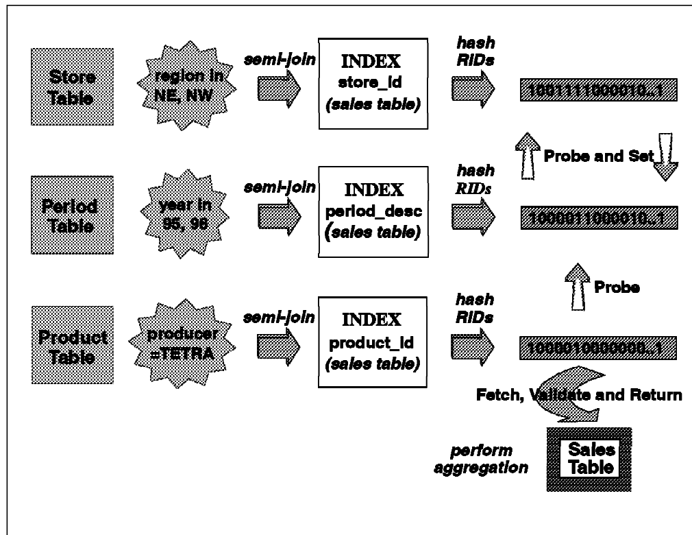
Figure 36. Star Join via DBIA
