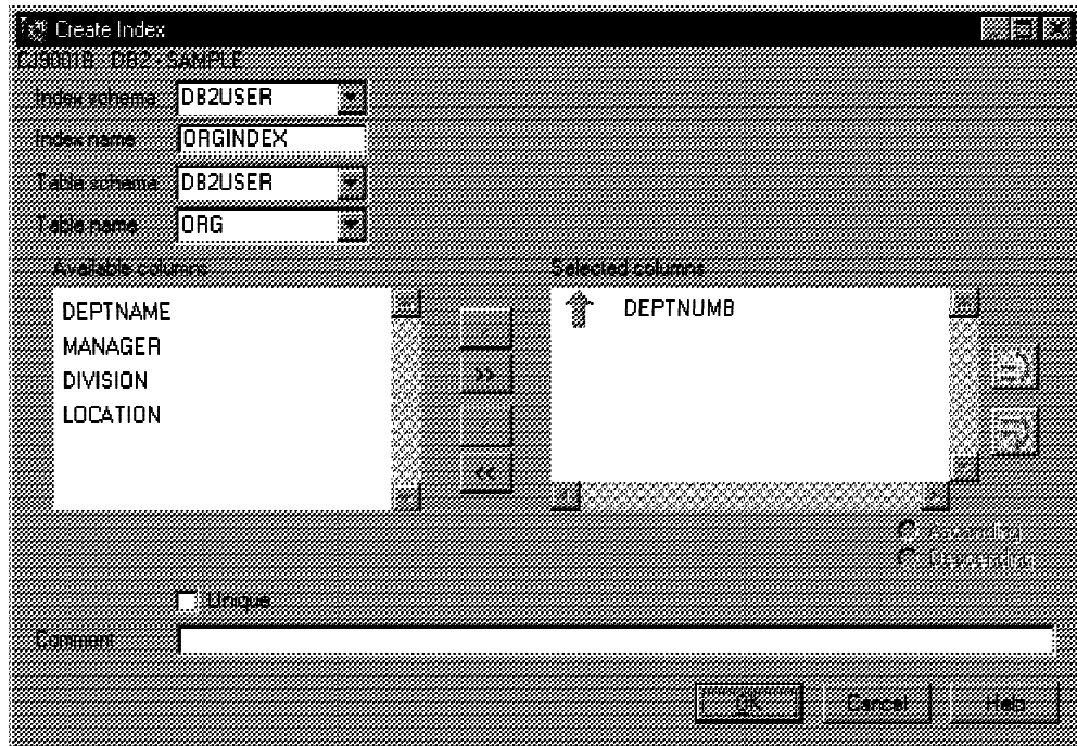
Figure 81. Create Index Notebook
