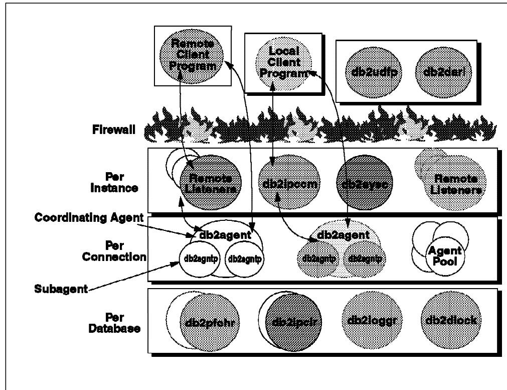
Figure 29. Process Model on SMP
