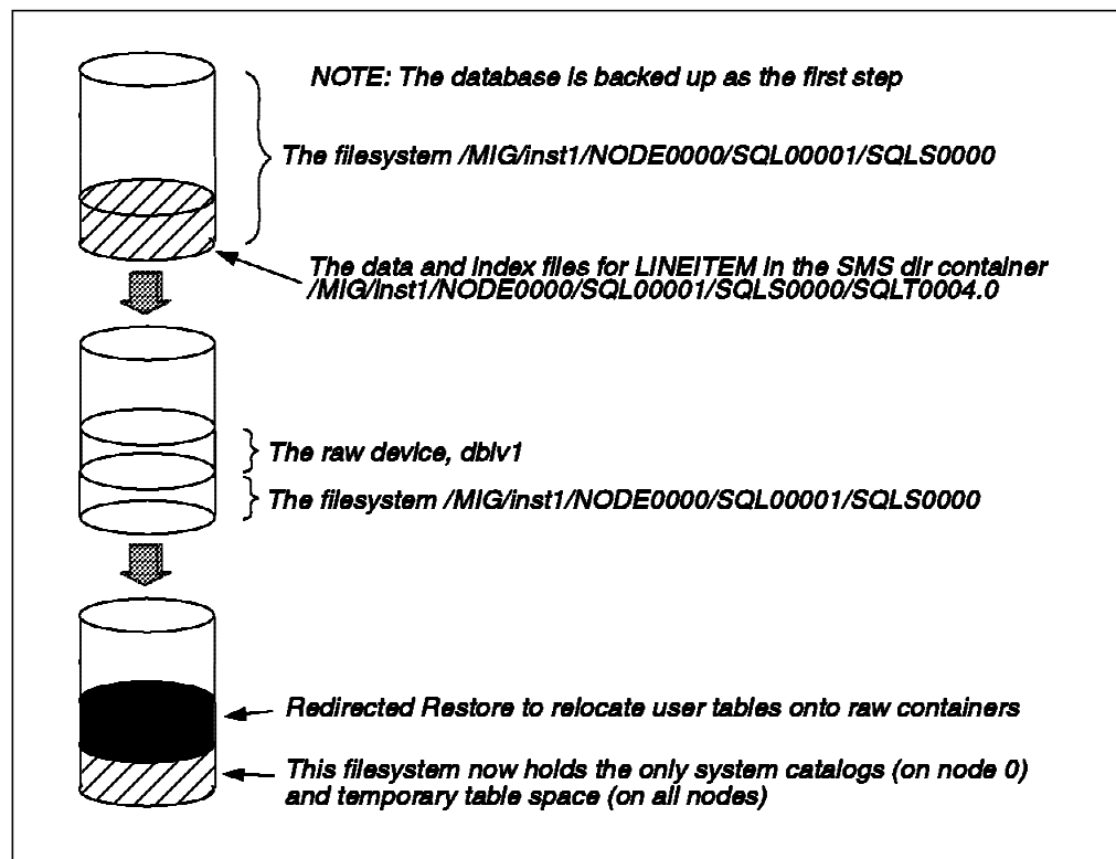
Figure 186. Redirected Restore Method
