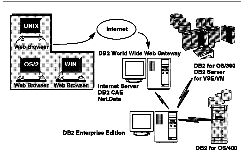
Figure 6. Accessing Data via the Internet
