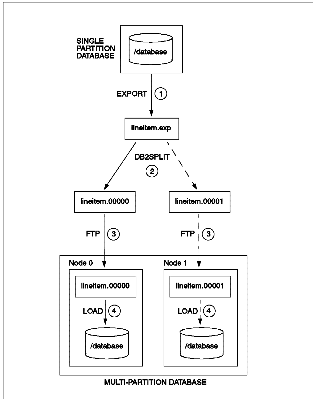
Figure 176. Moving Data to a Multi-Partition Database
