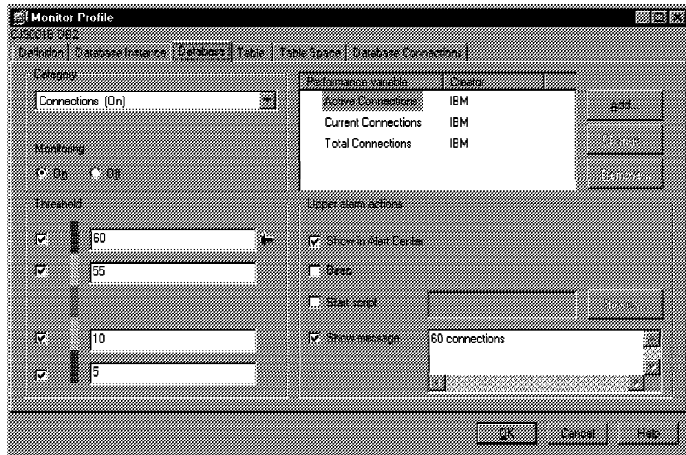
Figure 104. Performance Monitor Profile
