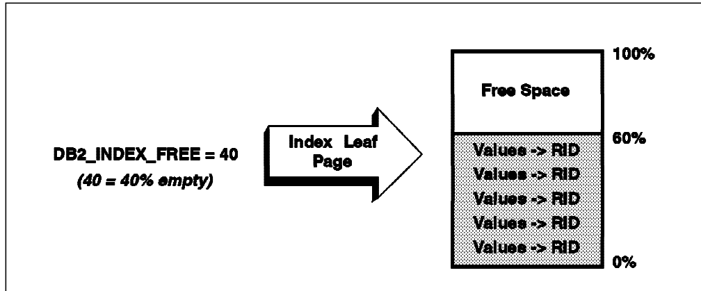
Figure 19. Index Free Space
