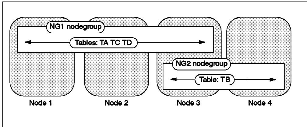
Figure 178. Example Scenario before Database Migration
