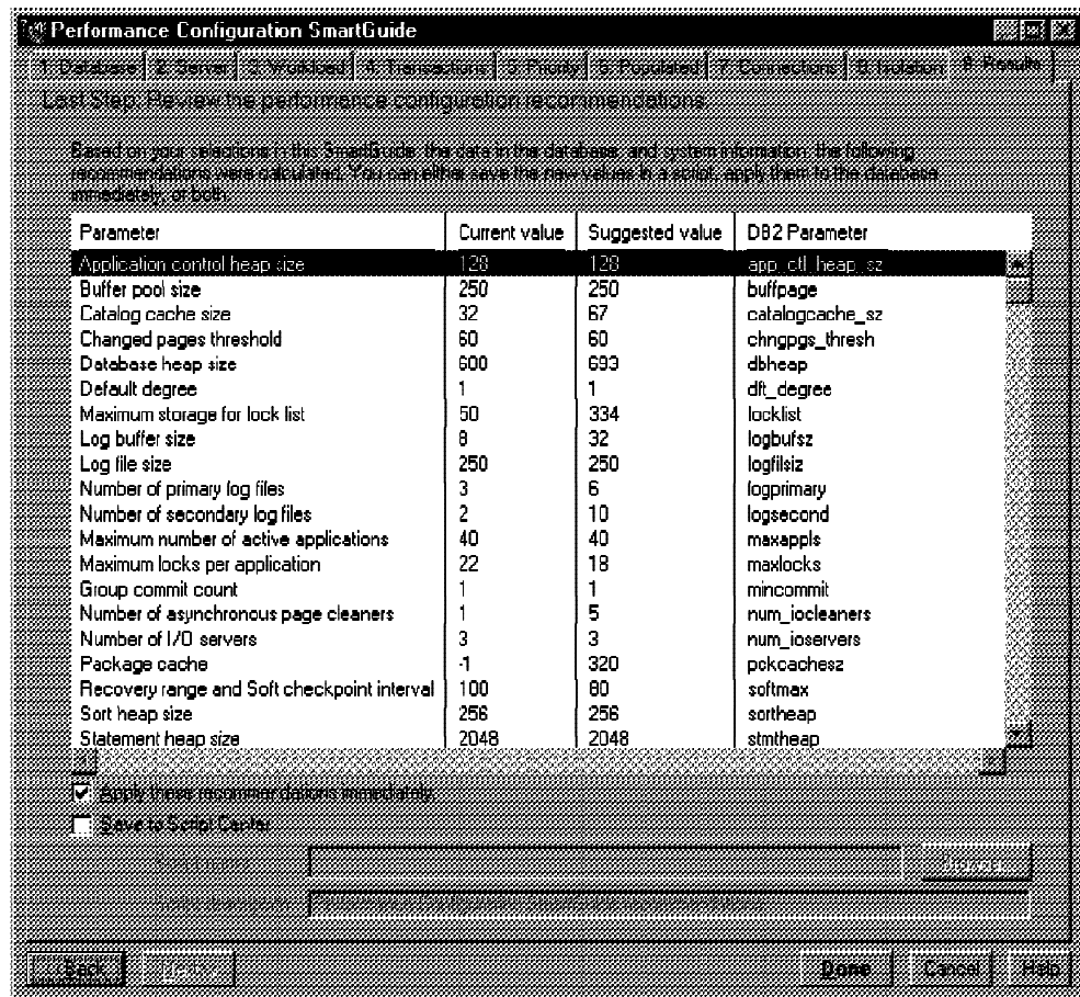
Figure 100. Performance Configuration SmartGuide - Results
