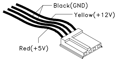
3.5-In. Diskette Drive Power Cable Connector
