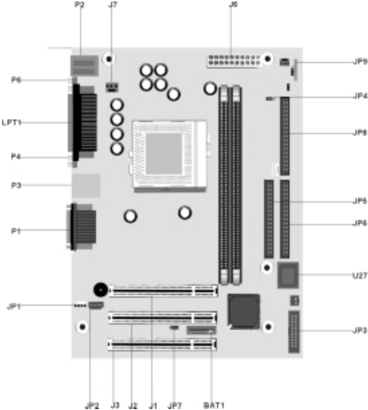
Jumpers and Connectors Locations on System Board for machine types 2255 and 2275
