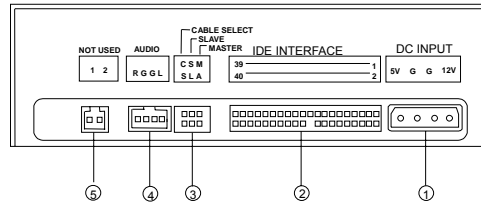
CD-ROM Rear Panel
