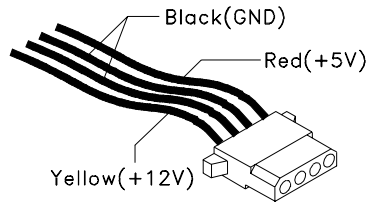
Hard Drive or CD-ROM Power Cable Connector
