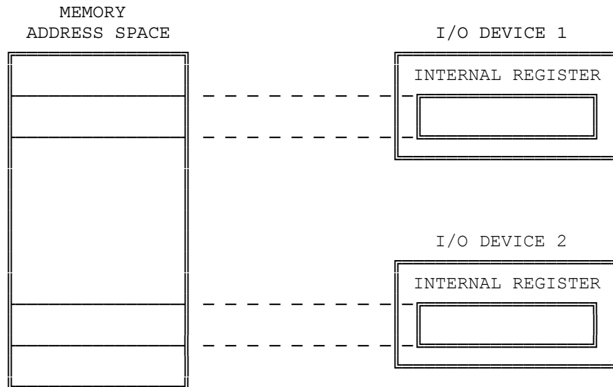
Figure 8-1. Memory-Mapped I/O
