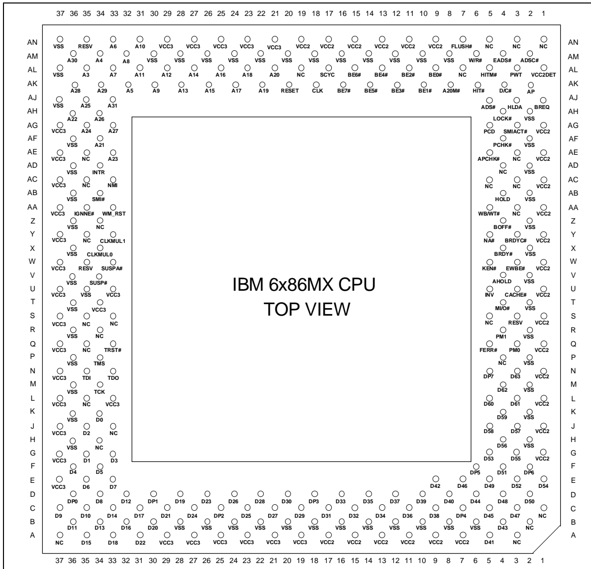
Figure 5-1. 296-Pin SPGA Package Pin Assignments
