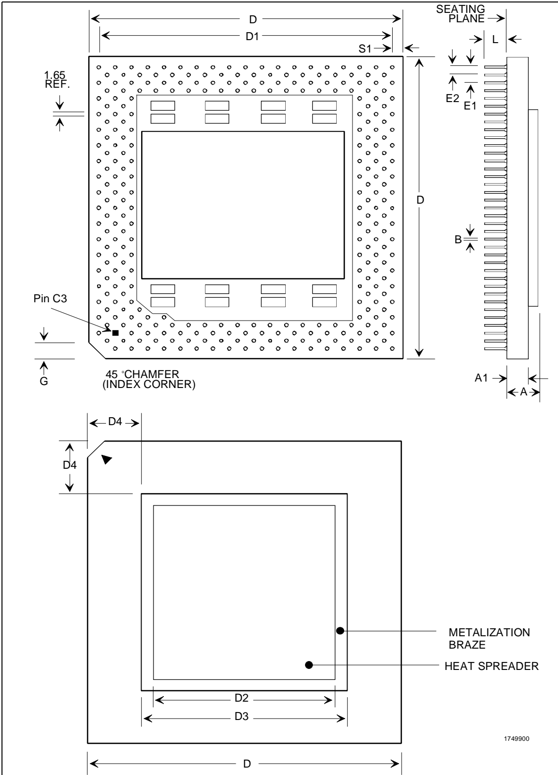
Figure 5-3. 296-Pin SPGA Package
