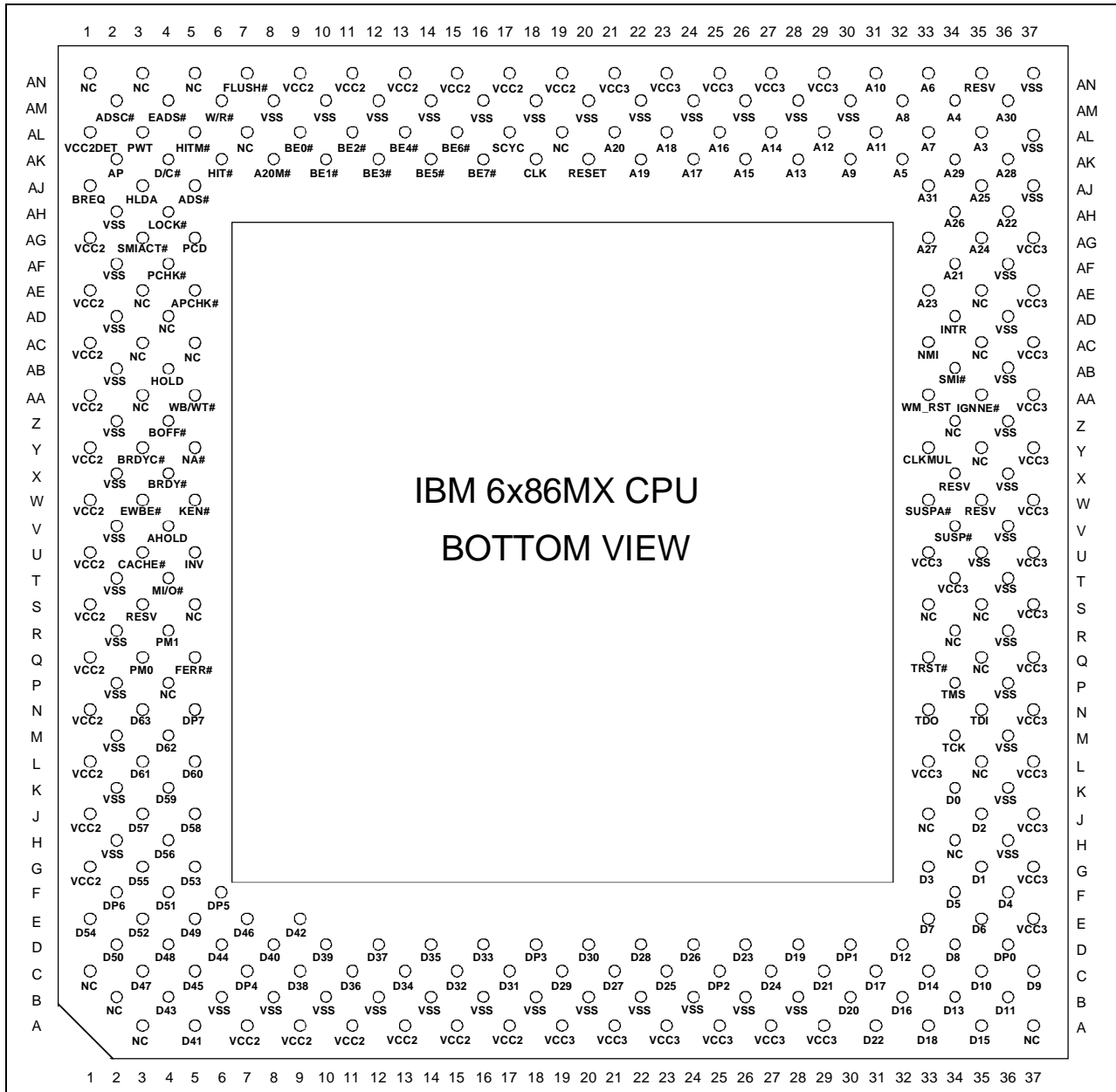
Figure 5-2. 296-Pin SPGA Package Pin Assignments (Bottom View)
