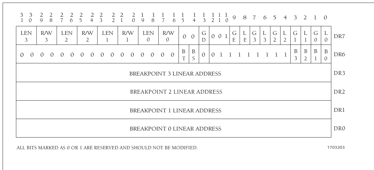
Figure 2-23. Debug Registers
