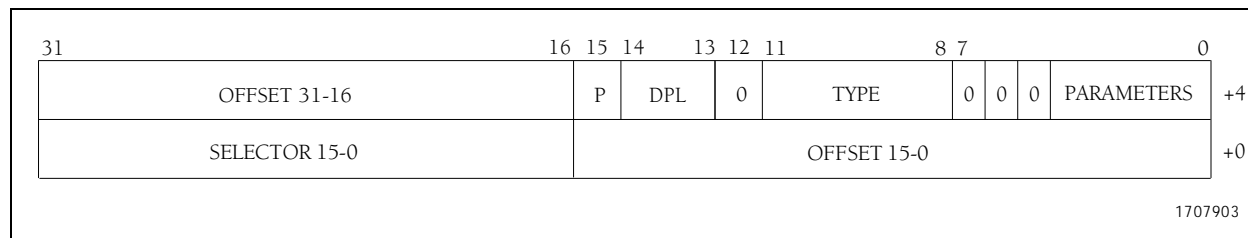
Figure 2-9. Gate Descriptor
