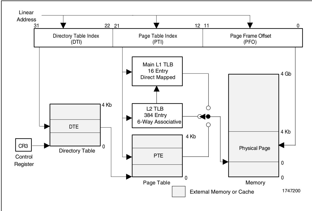
Figure 2-29. Paging Mechanism
