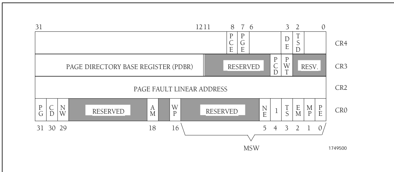
Figure 2-6. Control Registers
