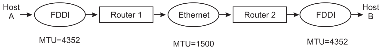
Figure 23. Inter-Subnet Fragmentation. This illustration shows a data path from Host A, through an FDDI with an MTU=4352, through Router 1, to the Ethernet with an MTU=1500. From there it goes to Router 2 and another FDDI with an MTU=4352 and out to Host B. An explanation of how fragmentation occurs in this example is described in the text immediately following the illustration.
