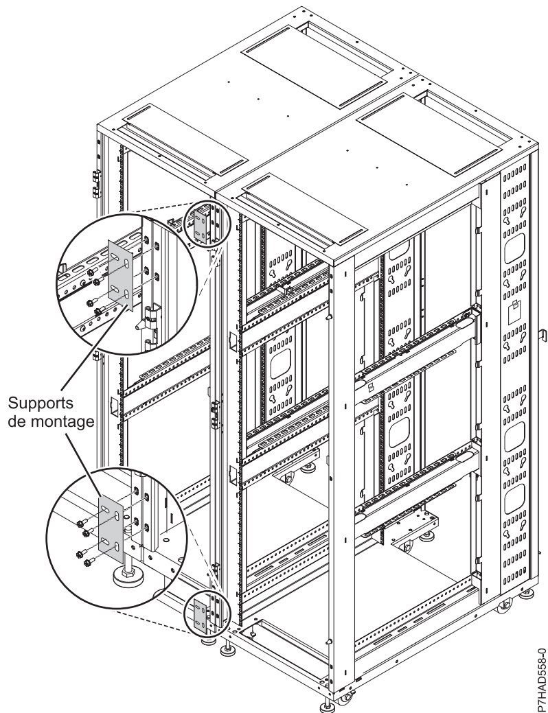
Figure 25. Supports de montage
