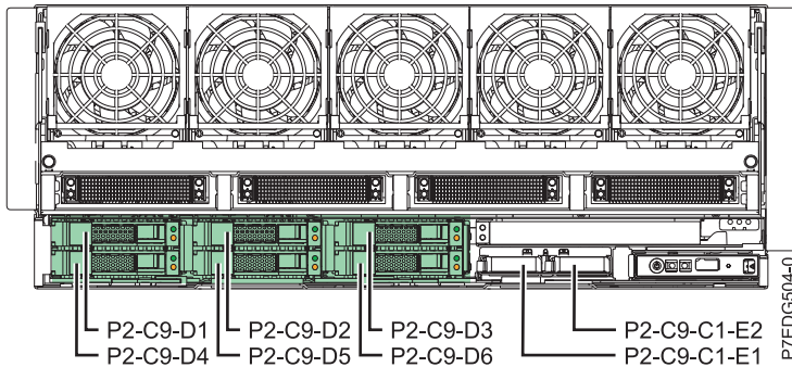
Figure 11. Disk bays controlled by both embedded SAS adapters when using dual storage IOA with internal drives
