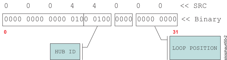
Figure 3. Decoding FRU 00044000
