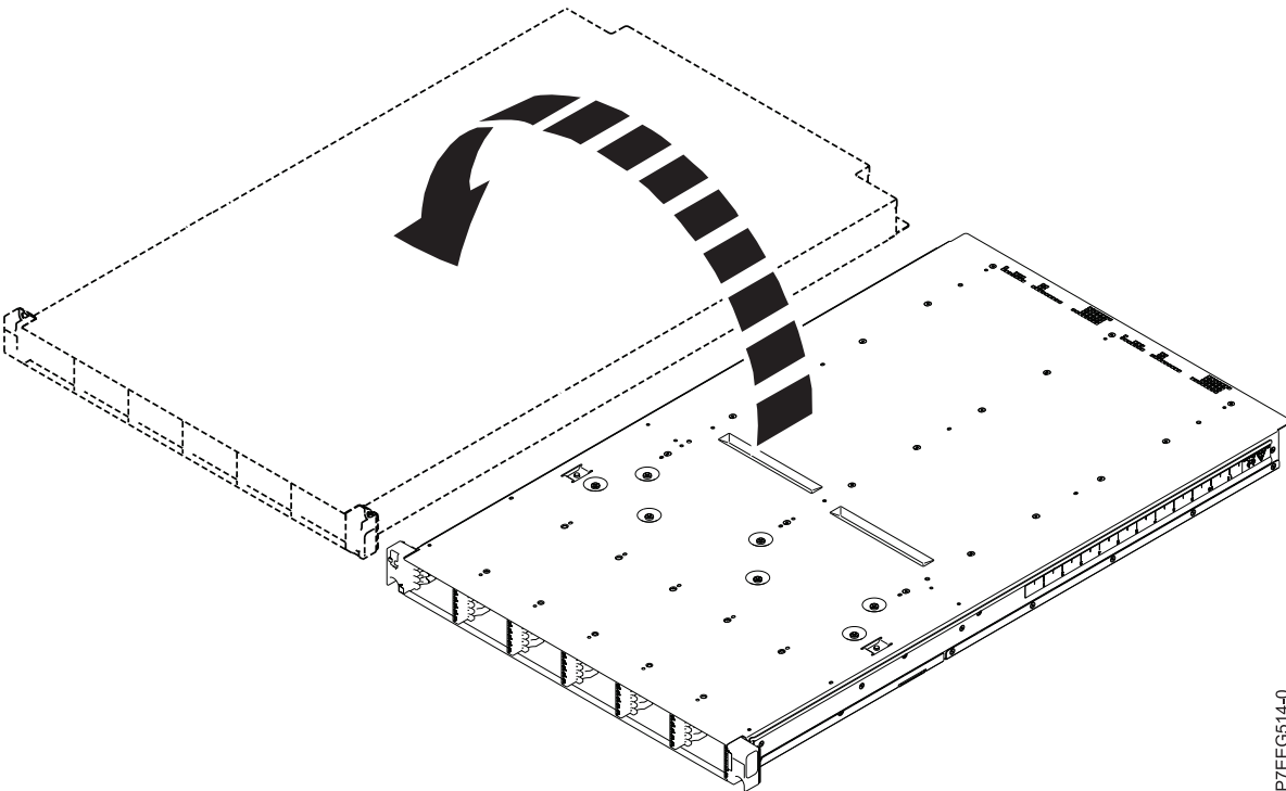
Figure 17. Turning the enclosure top side up
