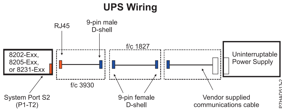
Figure 186. UPS wiring for the 02E/4B, 02E/4C, 05F/6B, 05E/6C, 31E/2B, 31E/1C, and 31E/2C
