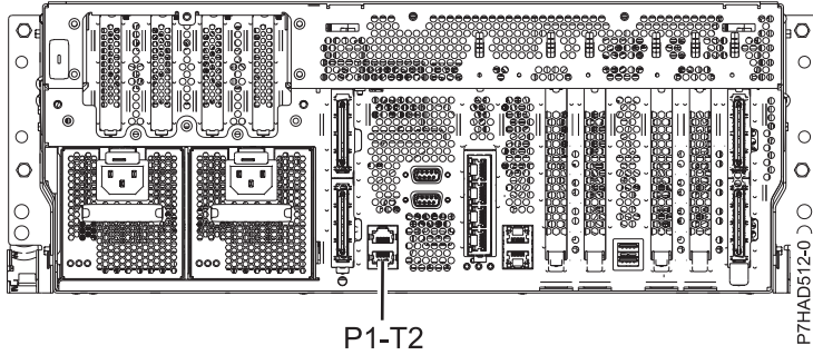
Figure 185. 02E/4B, 02E/4C, 05F/6B, and 05E/6C rear view with cable installation location
