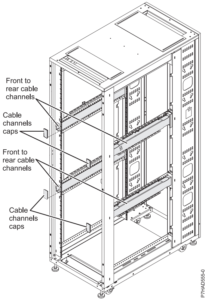
Figure 95. Cabling within the rack
