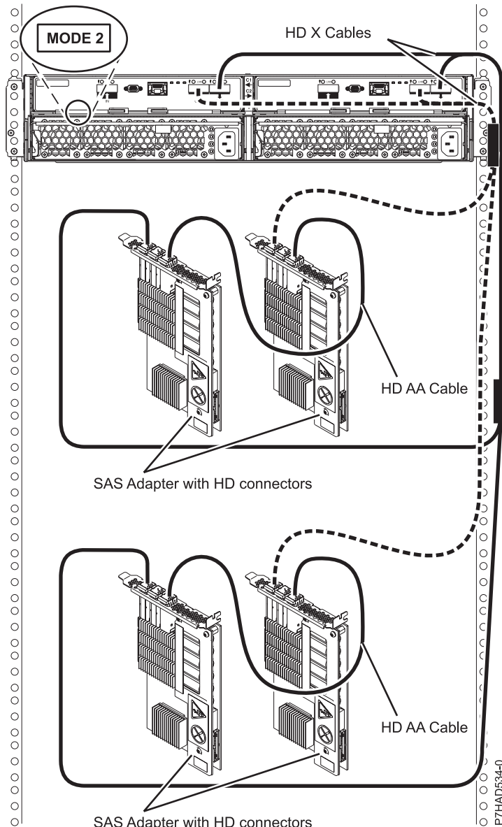
Figure 223. Mode 2 connection of a 58/87 drawer using HD connectors to two pairs of SAS adapters
