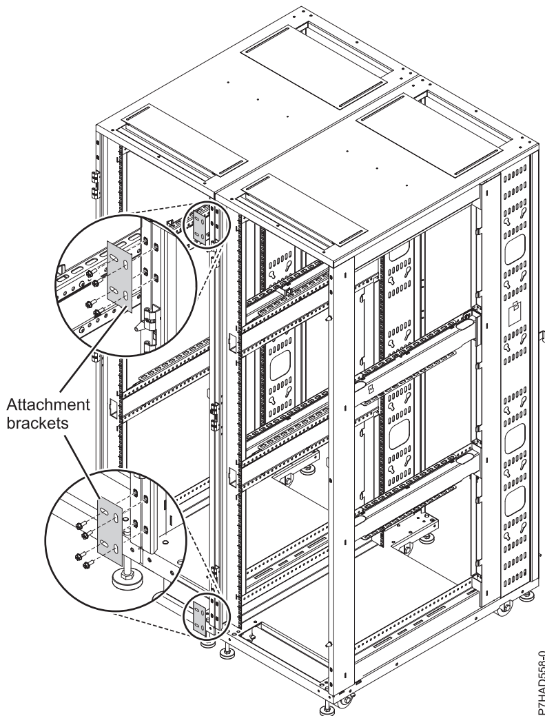
Figure 99. Attachment brackets
