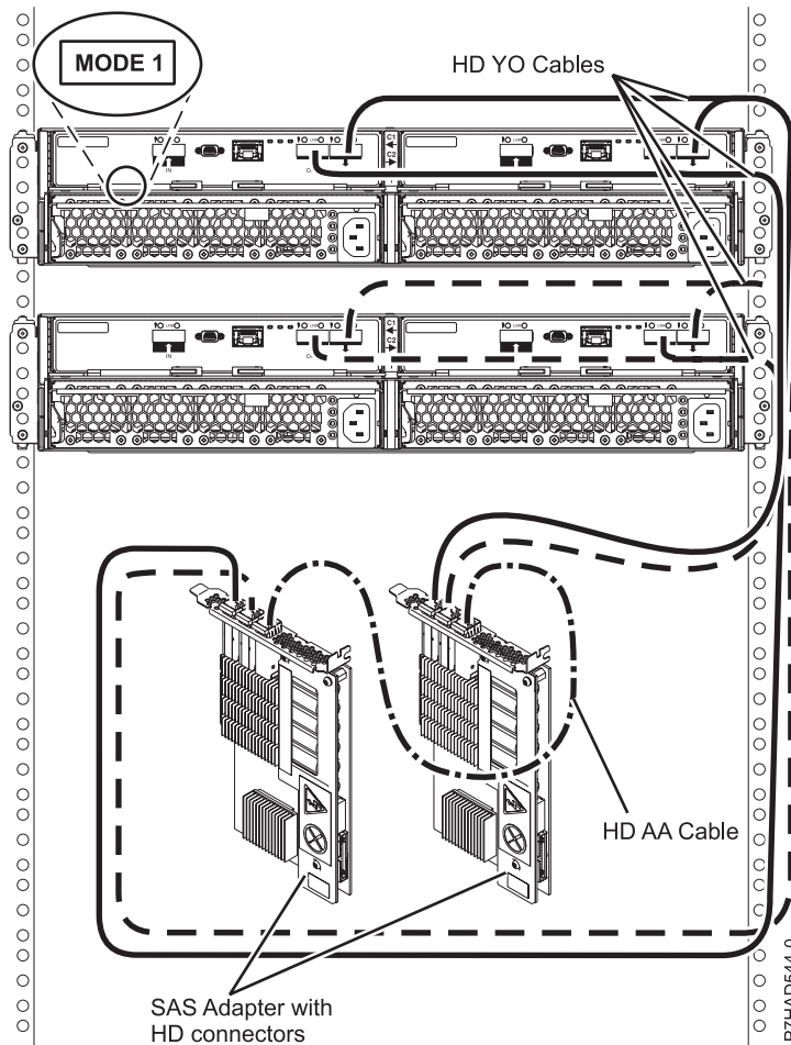
Figure 221. Mode 1 connection of two 58/87 drawers using HD connectors to two SAS adapters
