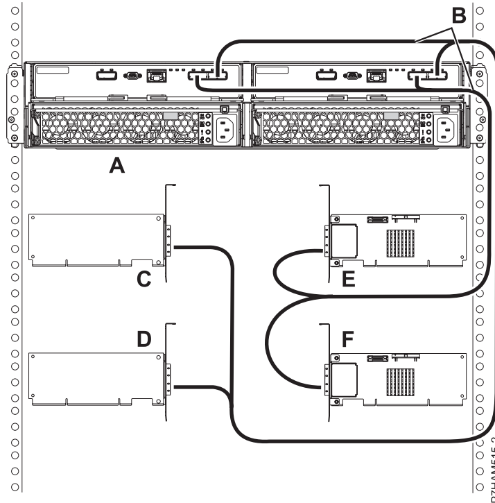
Figure 216. Mode 4 connection of a 58/87 drawer using X cables to quad SAS adapters
