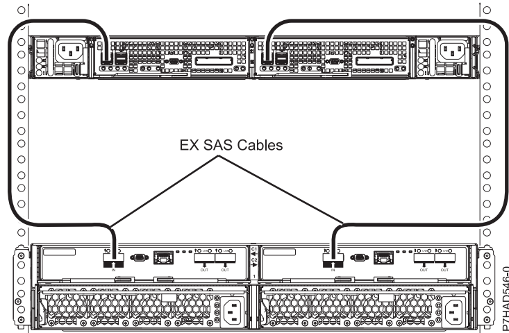
Figure 224. Connection of one 58/87 drawer by using HD EX cables to one EDR1
