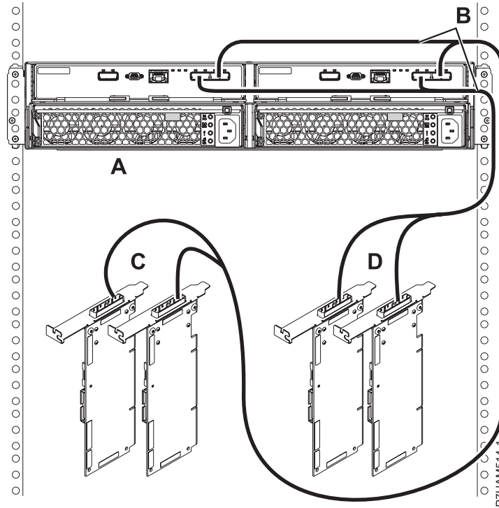
Figure 215. Mode 2 connection of a 58/87 drawer using X cables to quad SAS adapters (two pairs)
