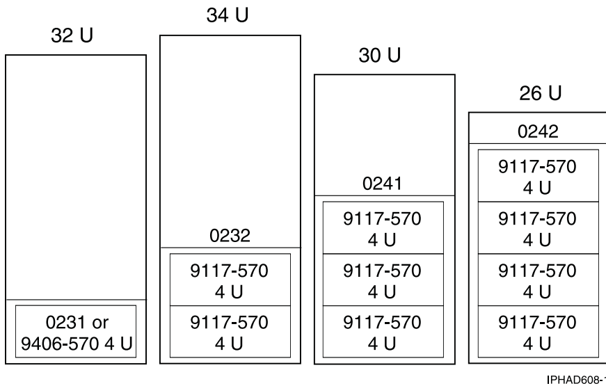
Figure 79. 5/70 in rack
