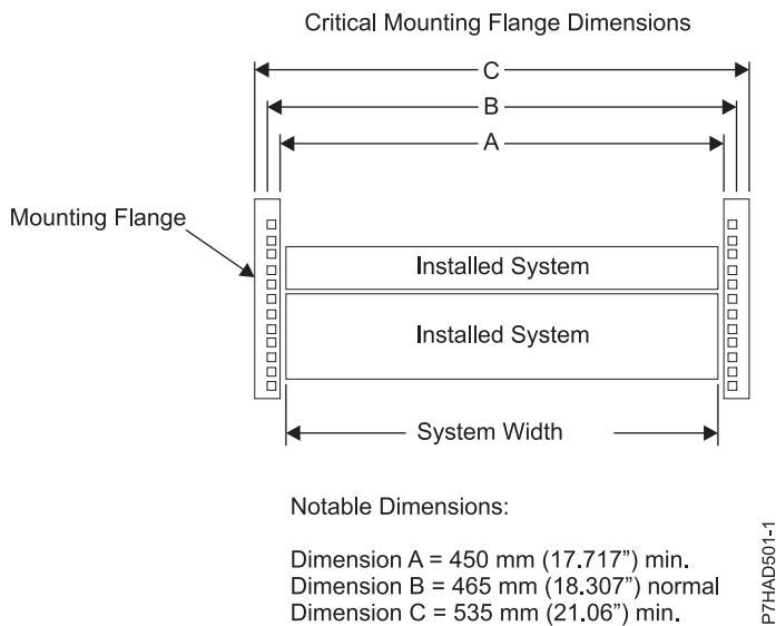
Figure 100. Critical mounting flange dimensions
