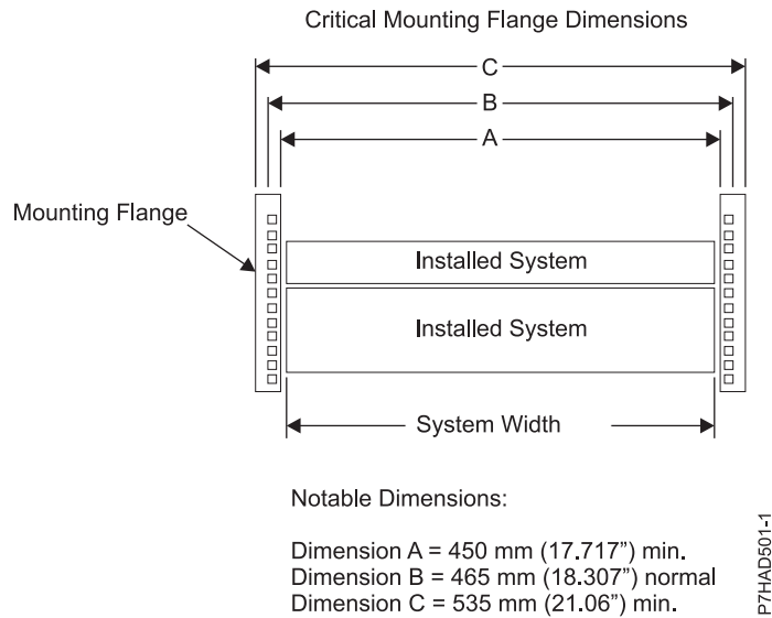
Figure 226. Critical mounting flange dimensions
