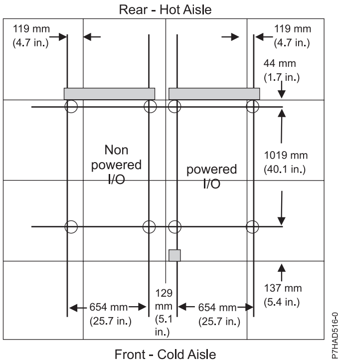
Figure 70. Rack placement for 600 mm (23.6 in.) tiles
