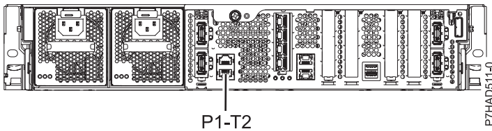
Figure 184. 31E/2B, 31E/1C, and 31E/2C rear view with cable installation location
