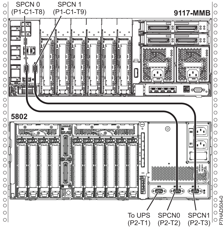
Figure 183. 17M/MB, 17M/MC, 79M/HB, and 79M/HC and 5208 or 5877 rear view cable installation location
