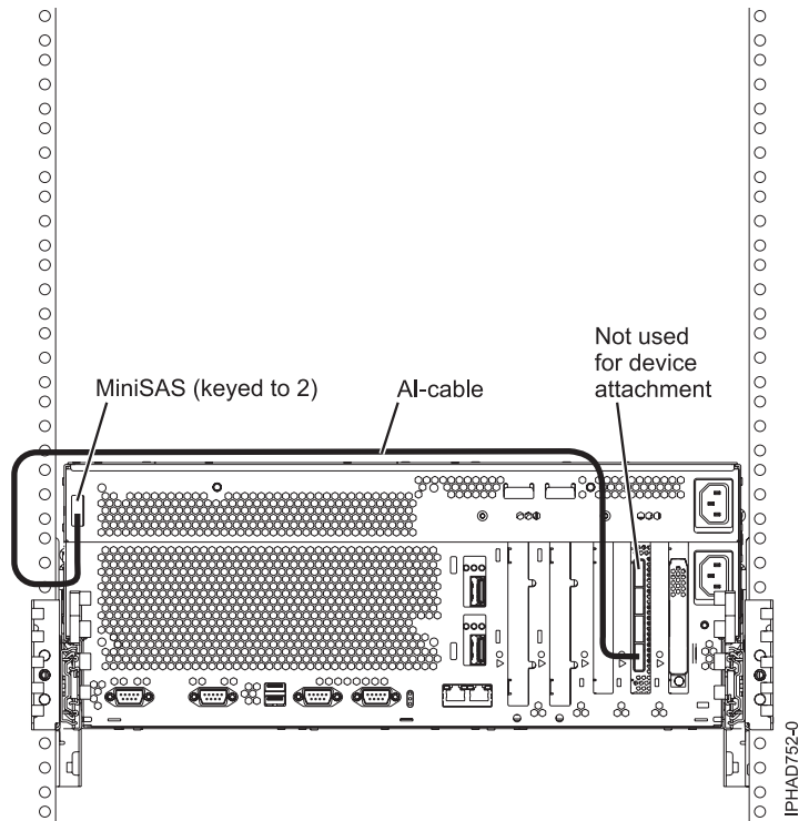
Figure 201. FC5904 or FC5908 adapter attached to disk expansion drawers
