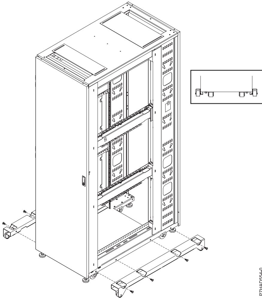
Figure 98. Outrigger locations
