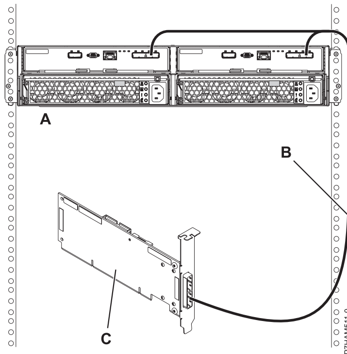
Figure 212. Mode 1 connection of a 58/87 drawer using a YO cable to a single SAS adaptor
