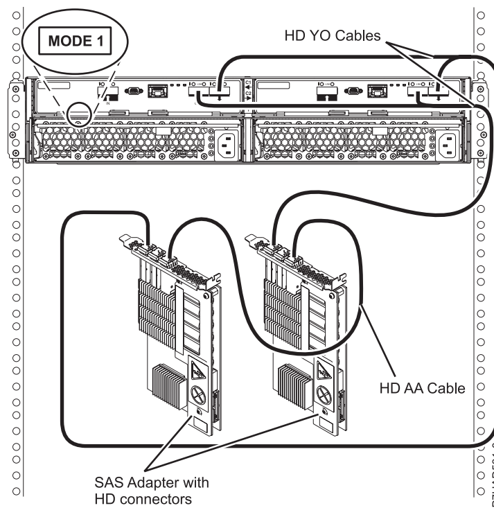
Figure 220. Mode 1 connection of a 58/87 drawer using HD connectors to two SAS adapters
