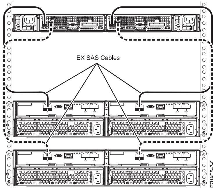
Figure 225. Connection of two 58/87 drawers by using HD EX cables to one EDR1
