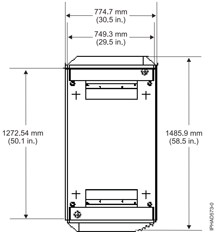
Figure 39. Plan view for single-frame systems with slimline doors
