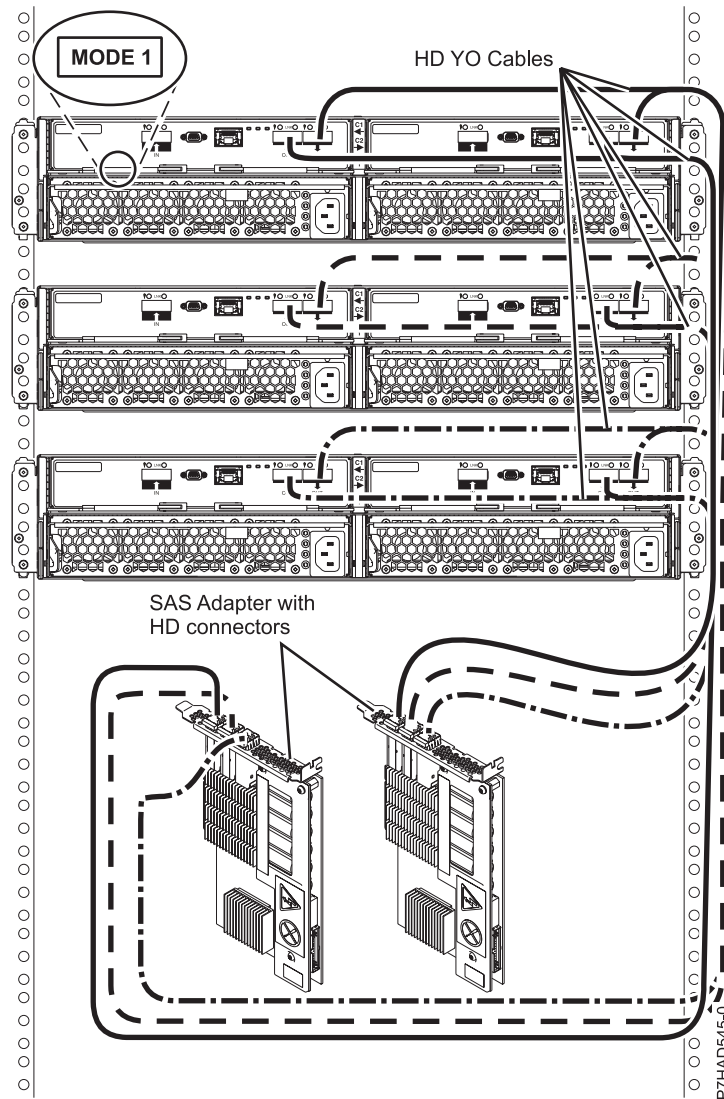
Figure 222. Mode 1 connection of three 58/87 drawers using HD connectors to two SAS adapters
