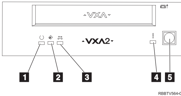
Figure 4. Front view of tape drive
