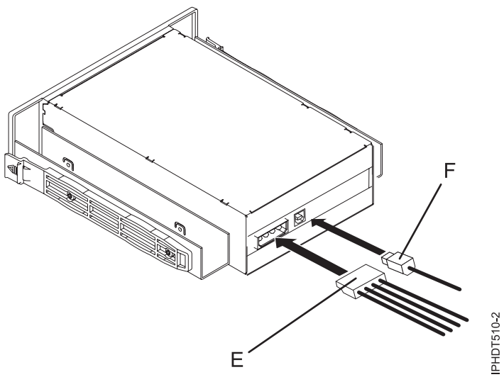
Figure 12. Internal drive, rear view, and connectors
