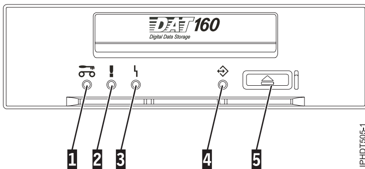
Figure 12. Front-view of tape drive
