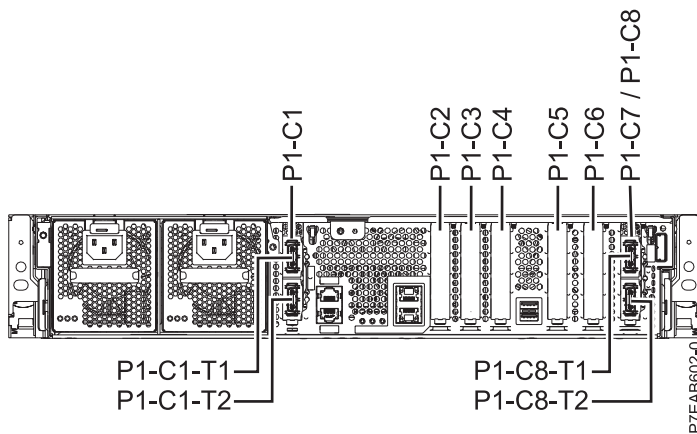
Figure 2. Rear view of the 31E/1C with location codes
