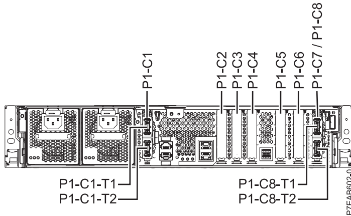
Figure 3. Rear view of the 31E/2C with location codes
