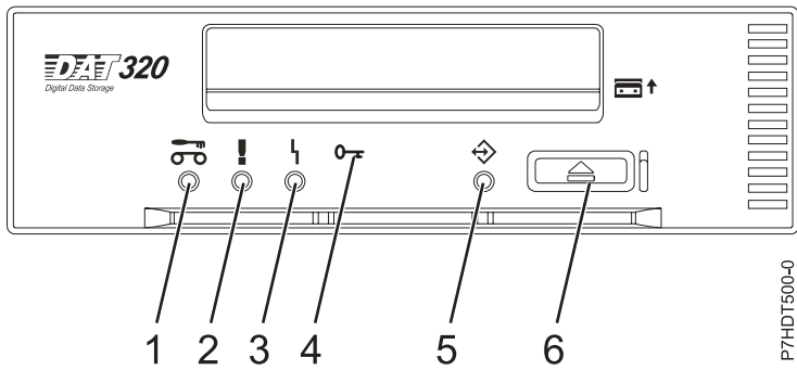
Figure 10. Front view of tape drive
