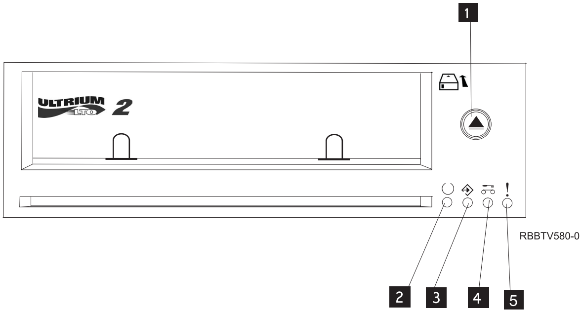
Figure 3. Front view of tape drive
