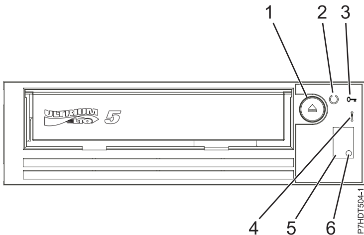
Figure 2. Front view of half-high LTO Drive
