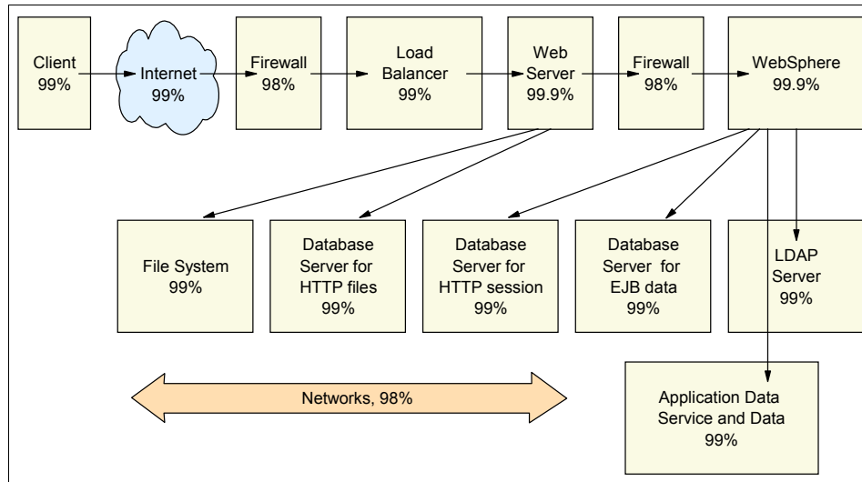
Figure 1-2 Availability chains
