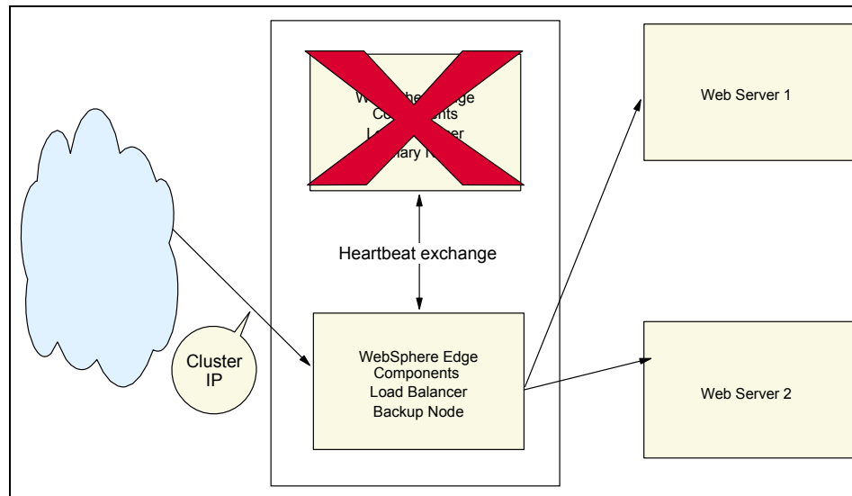
Figure 15-3 Load Balancer configuration after failover
