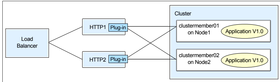
Figure 5-13 Single cell, single cluster topology - the details
