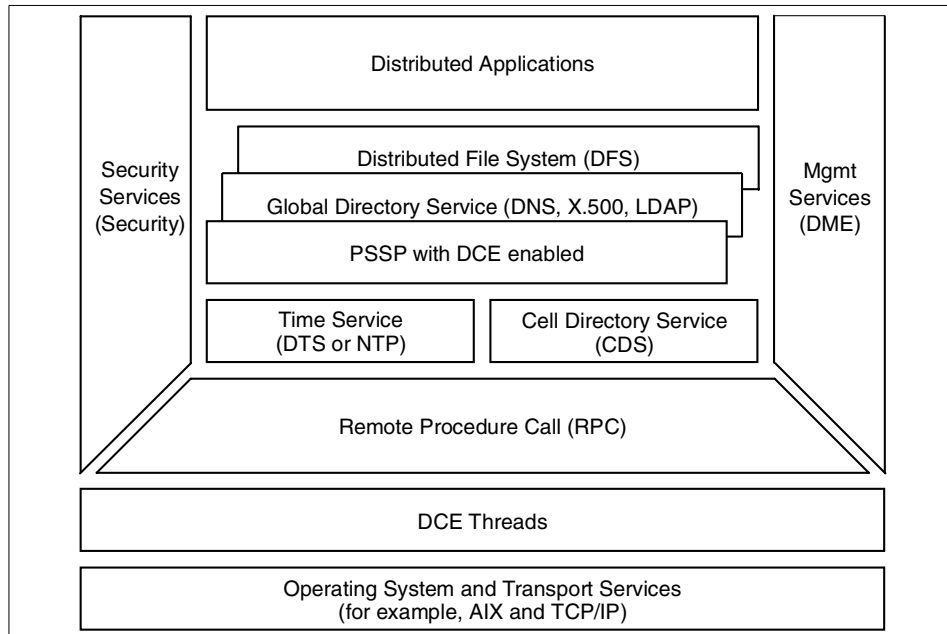
Figure 2. DCE architecture
