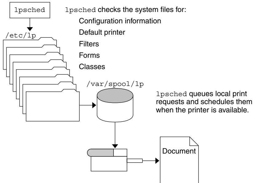
FIGURE 7-1 The lpsched Daemon Schedules Local Print Requests
