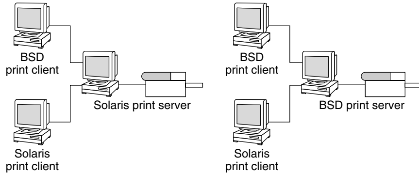
FIGURE 2-2 Solaris and lpd-Based Systems Print Configuration
