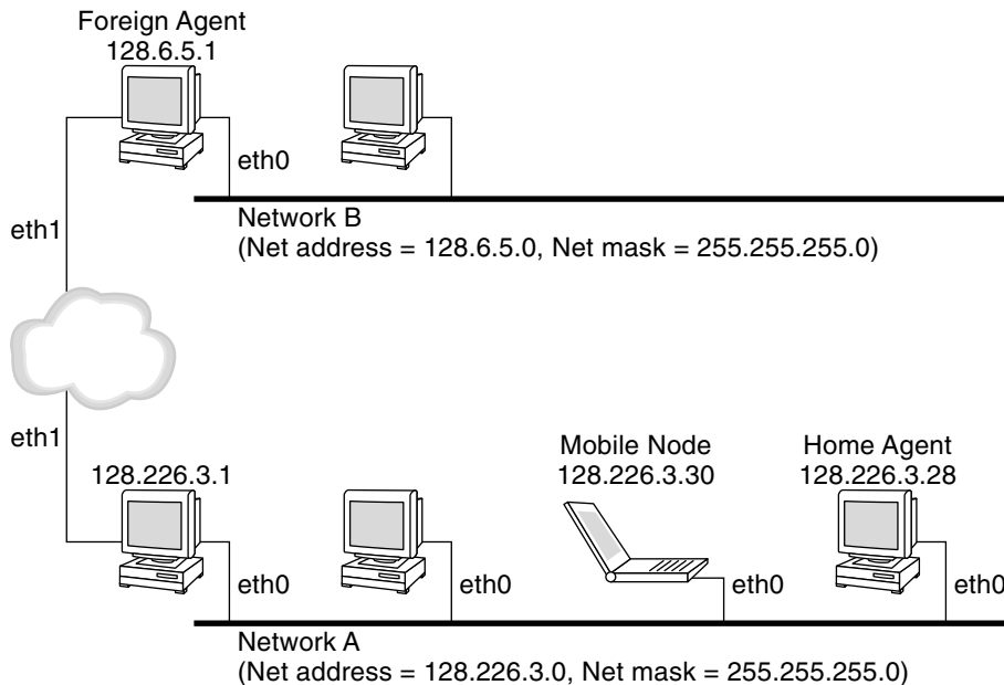
FIGURE 27-2 Mobile Node Residing on Home Network
