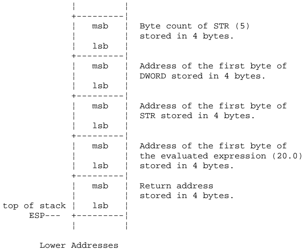
----- Figure 6-2. Stack After Call in Example A
