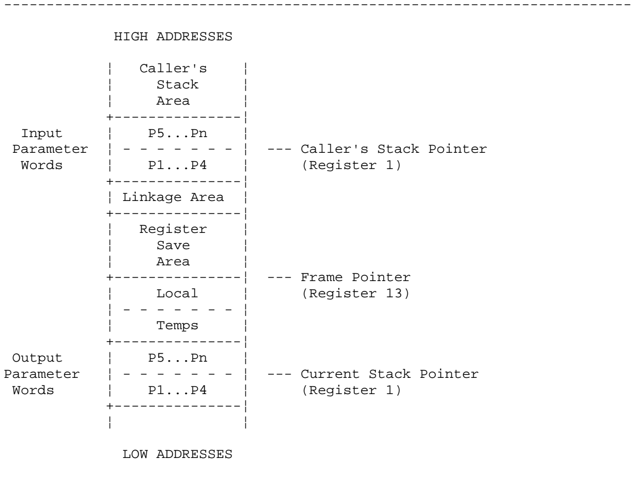
Figure 7-1. Contents of a Stack Frame
