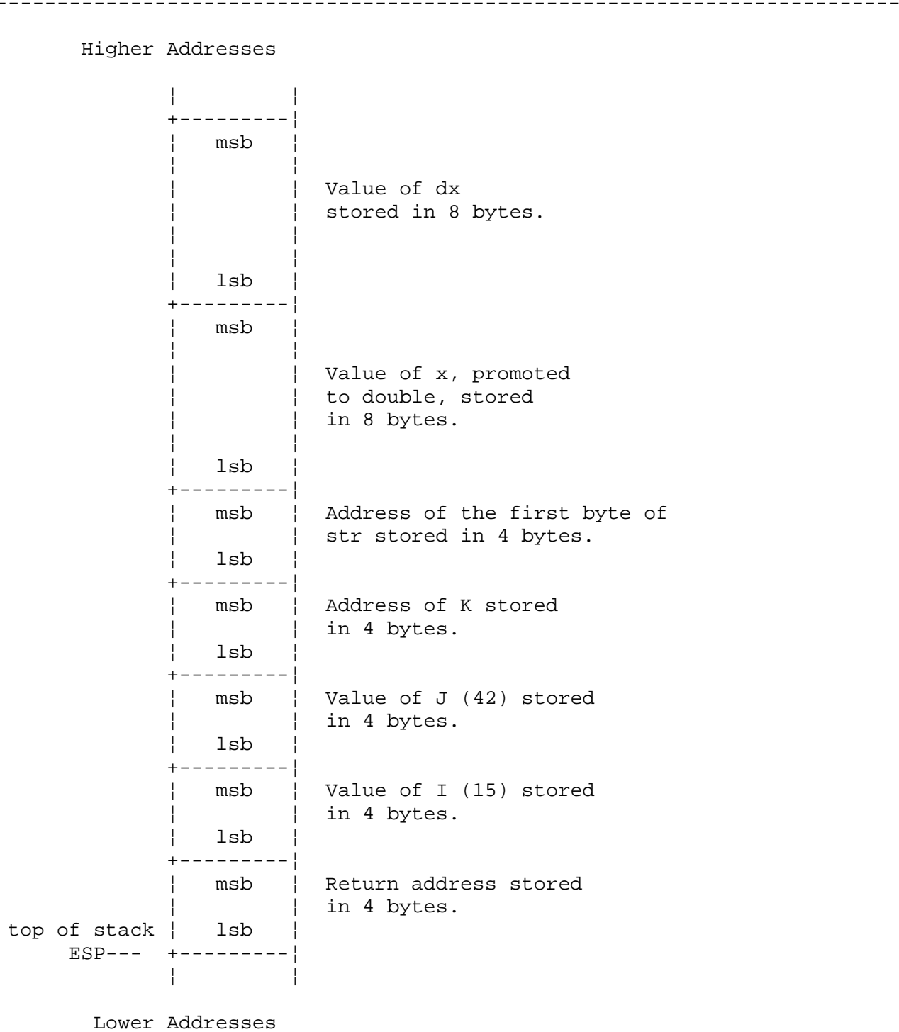
Figure 6-4. Stack After Call in Example E
