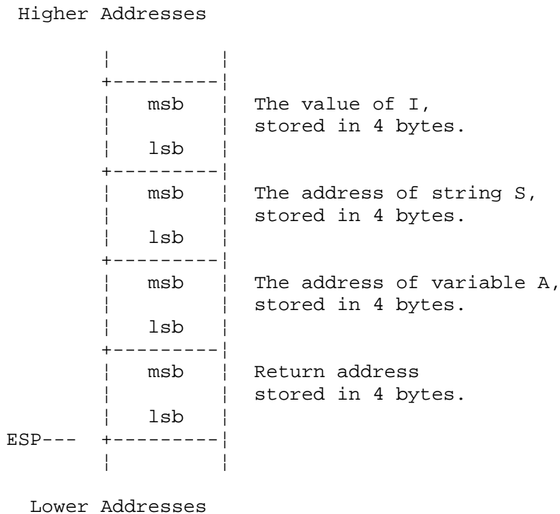
Figure 6-3. Stack After Call in Example C
