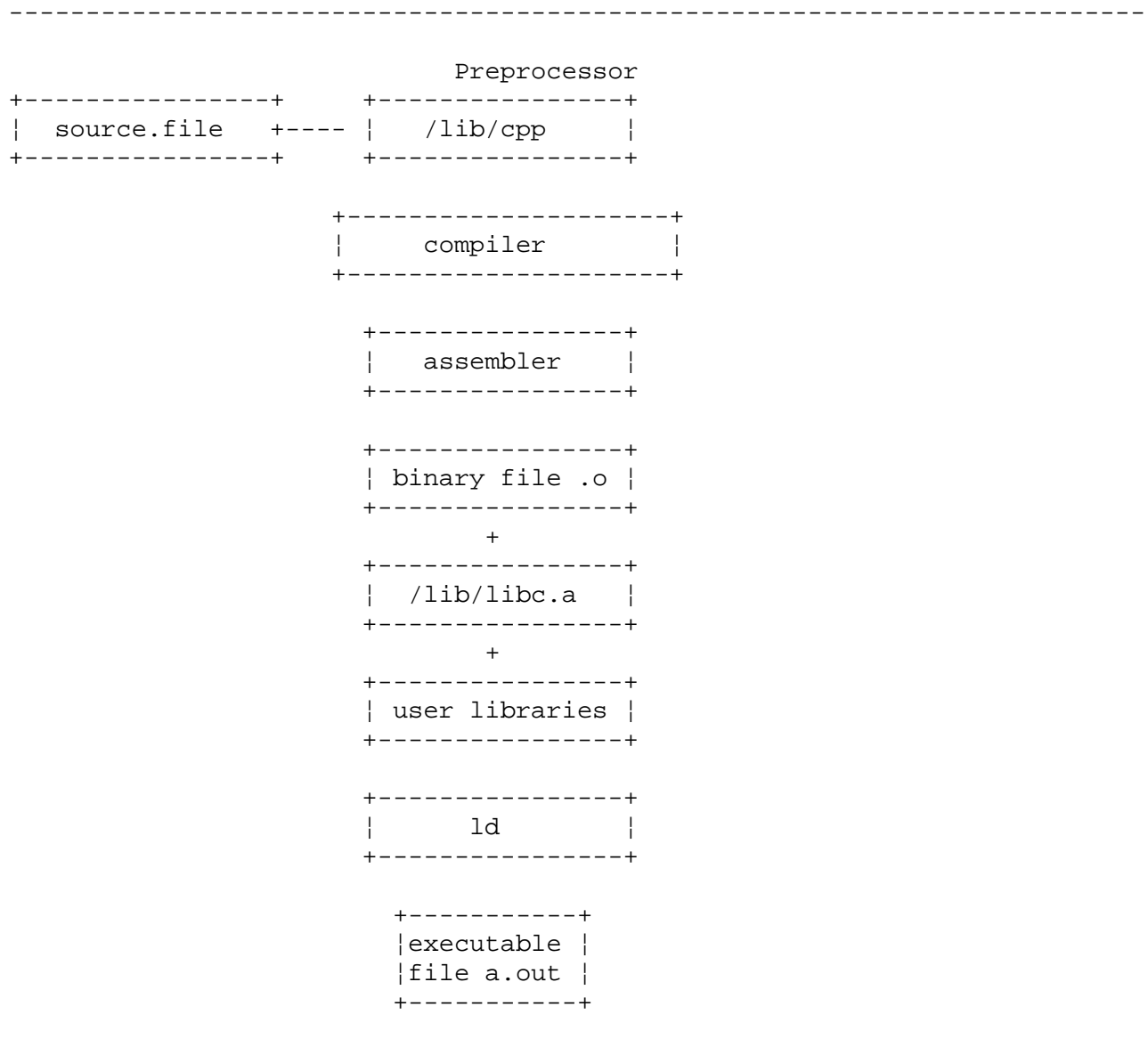
Figure 2-3. 370 and PS/2 MCC Compilation Process
