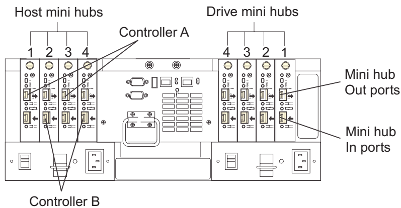
Figure 2. DS4500 Storage Subsystem ports and controllers
