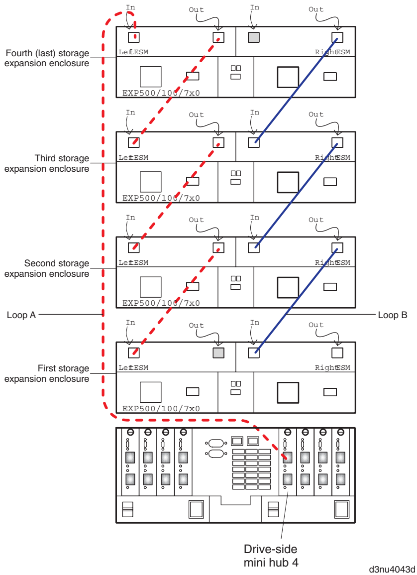
Figure 5. EXP100/700/710 storage enclosure
