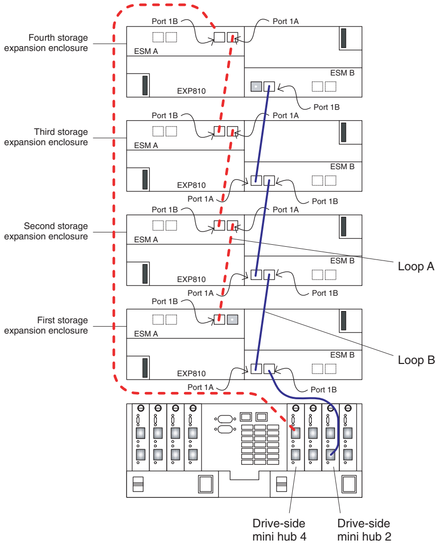
Figure 6. EXP 810 storage expansion enclosure
