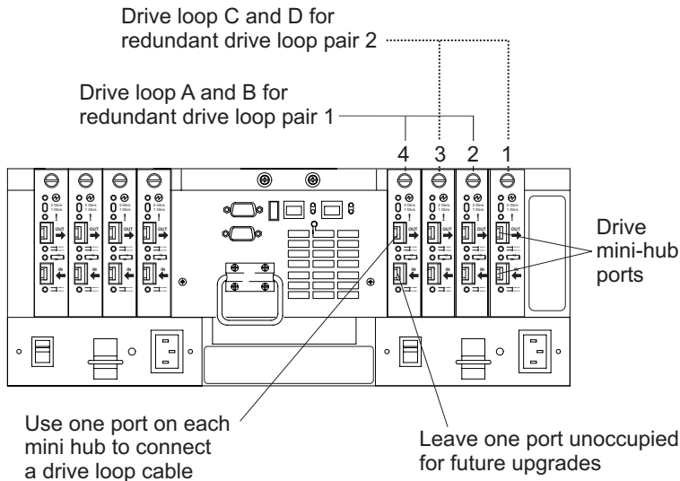
Figure 4. Drive mini-hub ports
