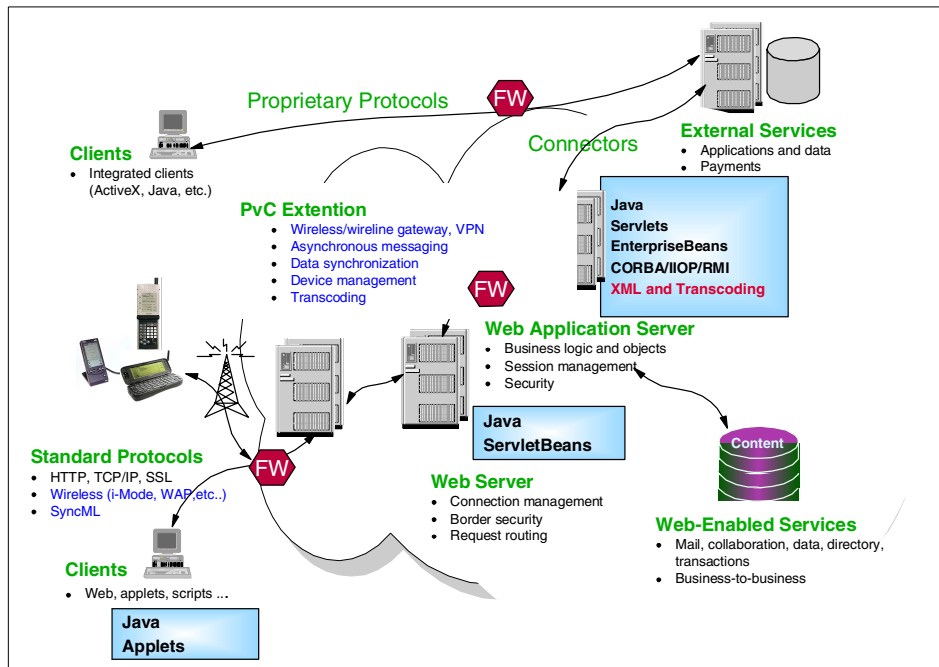
Figure 7. e-business environment with PvC devices
