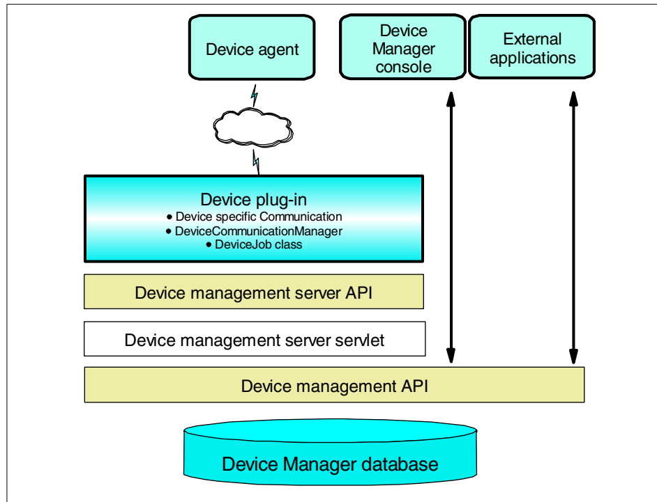
Figure 80. DMS components
