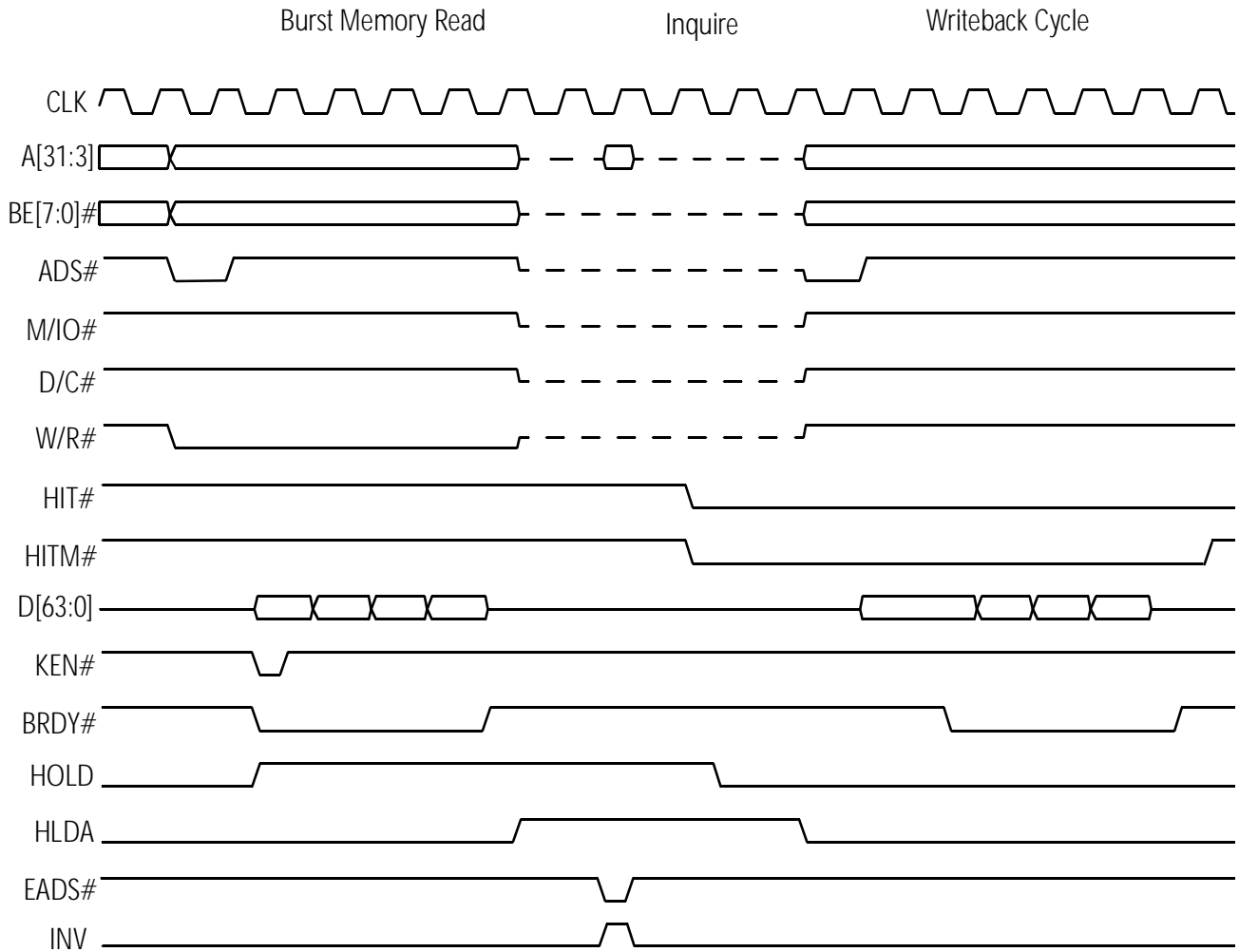
Figure 63. HOLD-Initiated Inquire Hit to Modified Line
