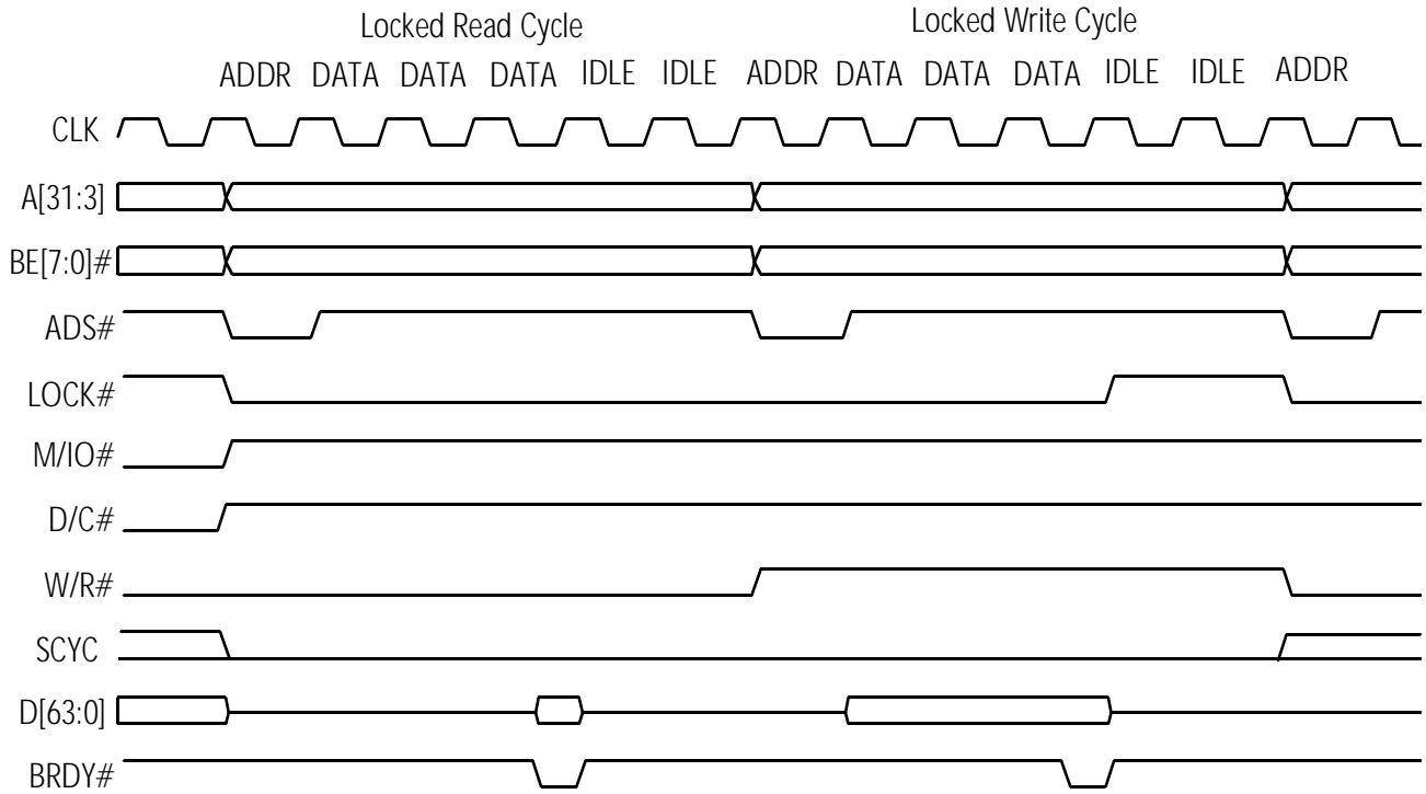
Figure 69. Basic Locked Operation
