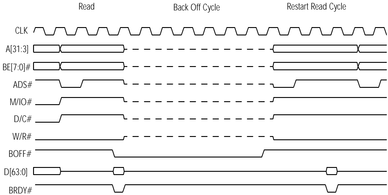
Figure 68. BOFF# Timing
