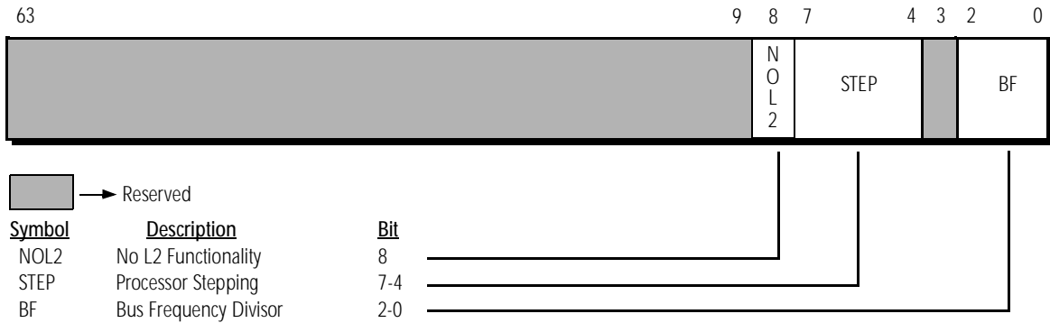
Figure 50. Processor State Observability Register (PSOR)
