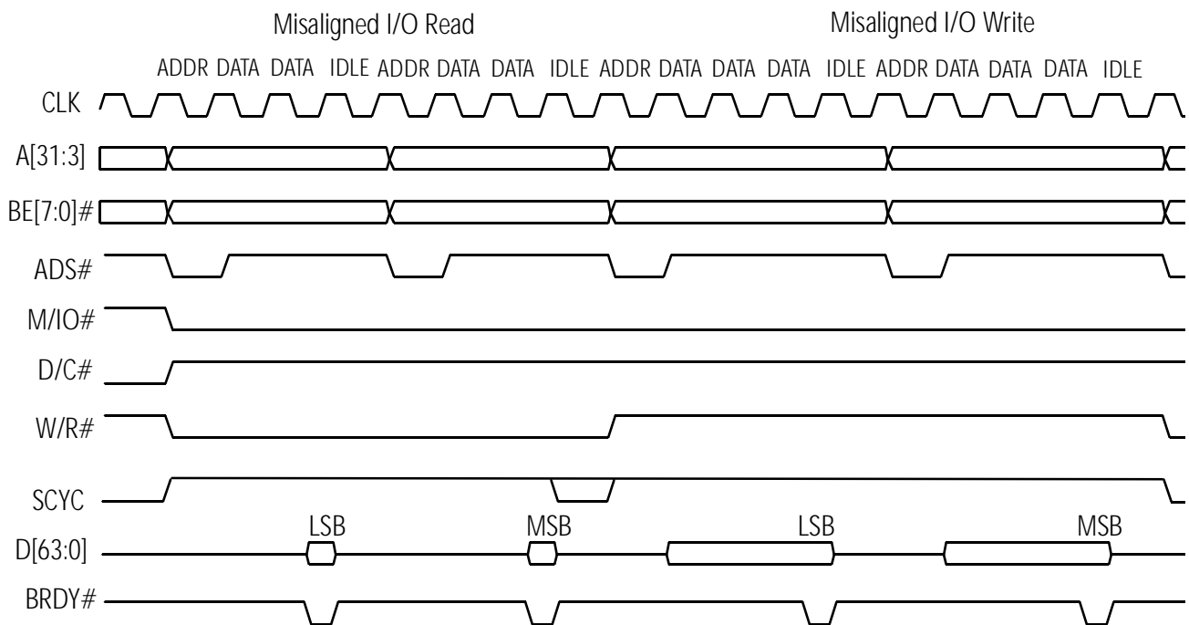
Figure 60. Misaligned I/O Transfer
