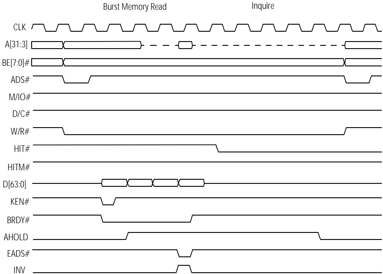
Figure 65. AHOLD-Initiated Inquire Hit to Shared or Exclusive Line
