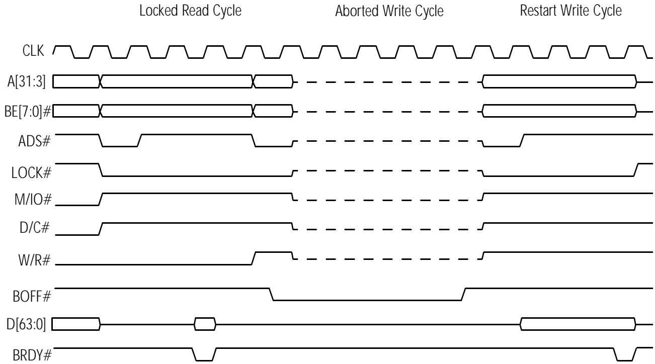
Figure 70. Locked Operation with BOFF# Intervention
