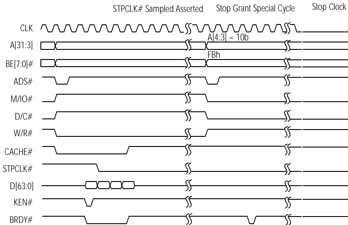
Figure 74. Stop Grant and Stop Clock Modes, Part 1
