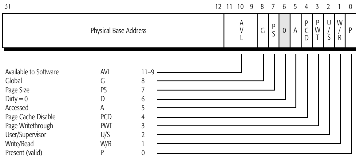
Figure 1-4. Page-Directory Entry (PDE)
