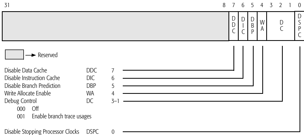
Figure 4-1. Hardware Configuration Register (HWCR)
