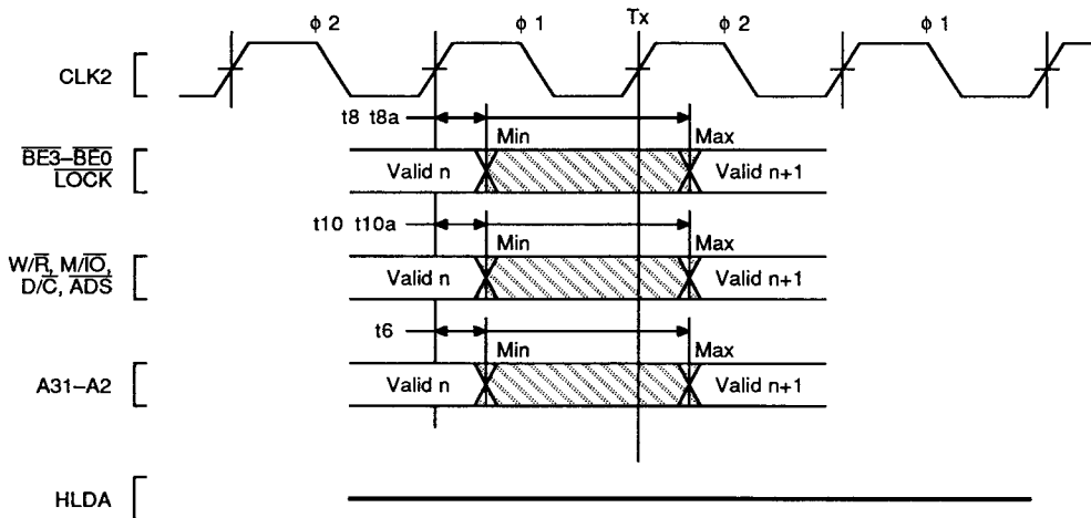
Figure 5. Output Valid Delay Timing
