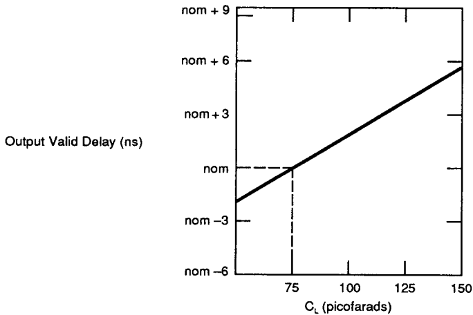
Figure 9. Typical Output Valid Delay Versus Load Capacitance at Maximum Operating Temperature ( C_L = 120 pF)
