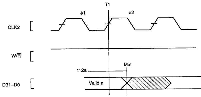
Figure 7. Write Data Hold Timing (25, 33, and 40 MHz)
