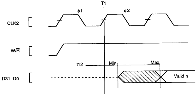
Figure 6. Write Data Valid Delay Timing (25, 33, and 40 MHz)
