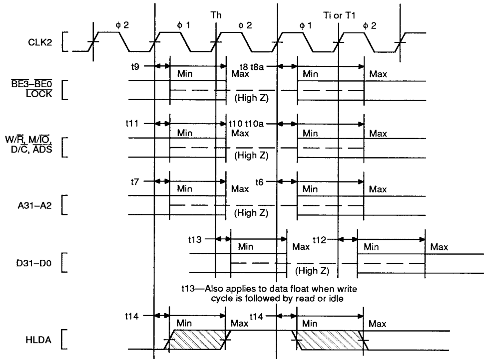
Figure 13. Output Float Delay and HLDA Valid Delay Timing
