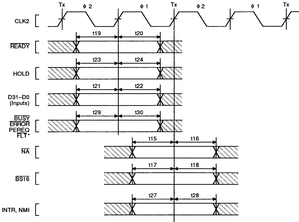
Figure 4. Input Setup and Hold Timing
