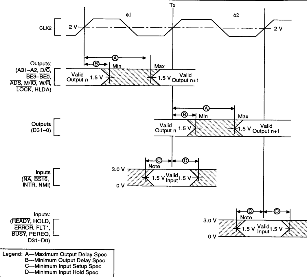
Figure 1. Drive Levels and Measurement Points
