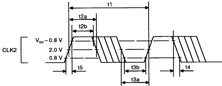
Figure 3. CLK2 Timing
