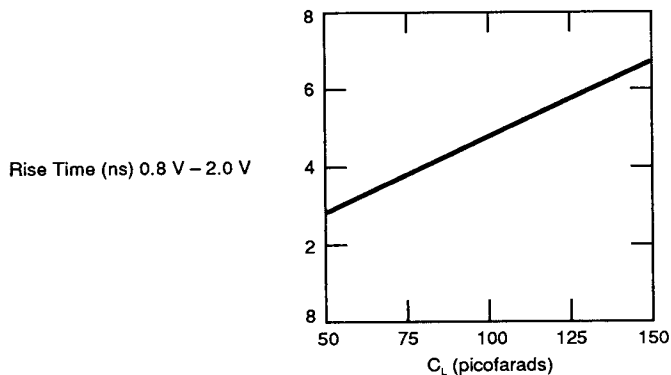
Figure 12. Typical Output Rise Time Versus Load Capacitance at Maximum Operating Temperature
