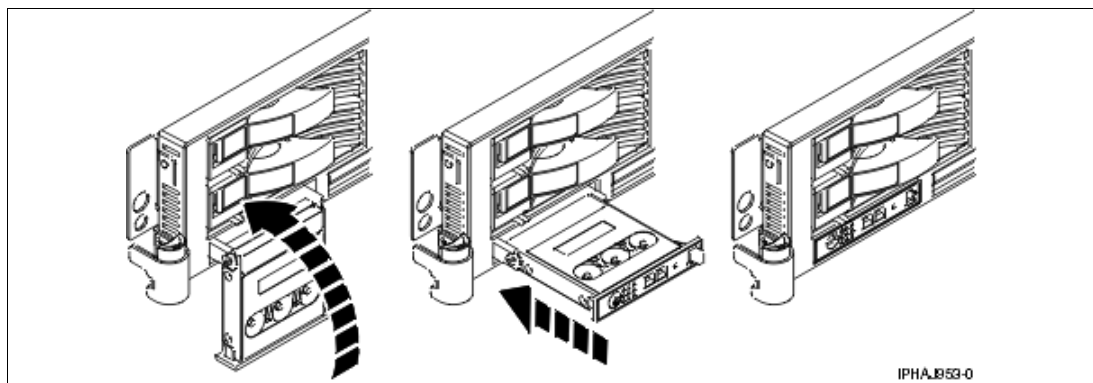
Figure 2-11 Restoring the p5-510 server control panel
