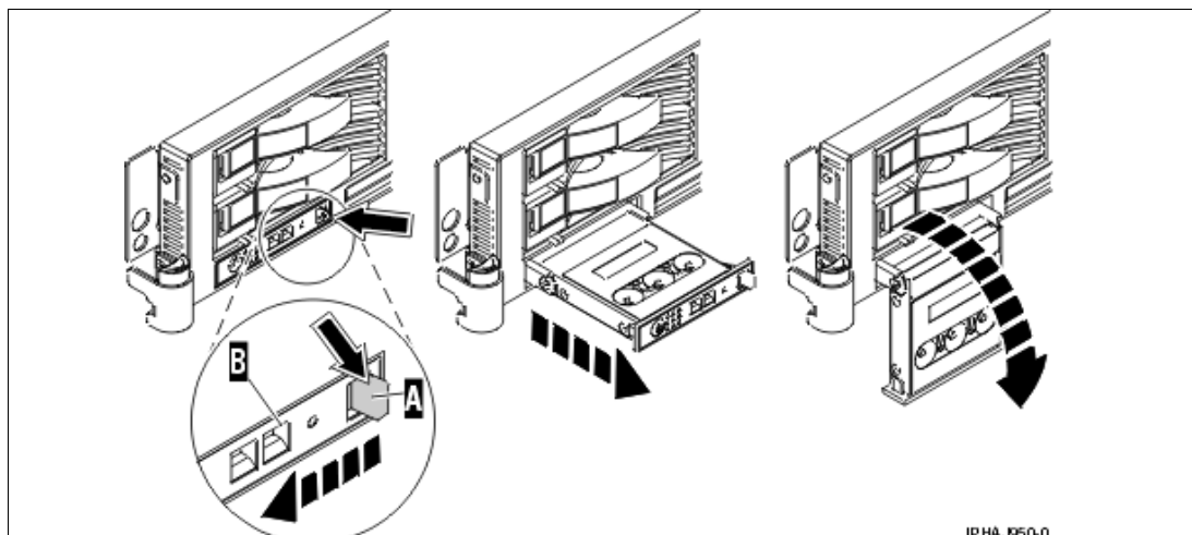
Figure 2-10 Accessing to the p5-510 server control panel
