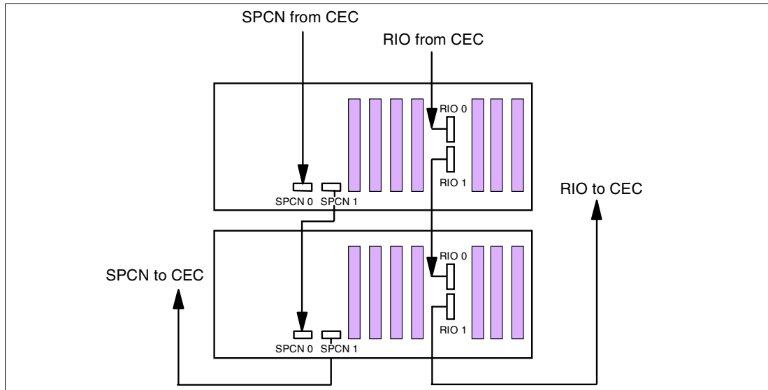
Figure 2-7 Remote I/O and SPCN cabling
