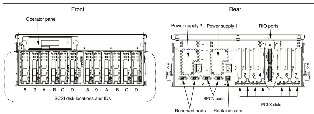
Figure 1-2 Views of 7311-D20 I/O drawer
