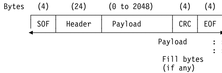
Figure 74. General frame format
