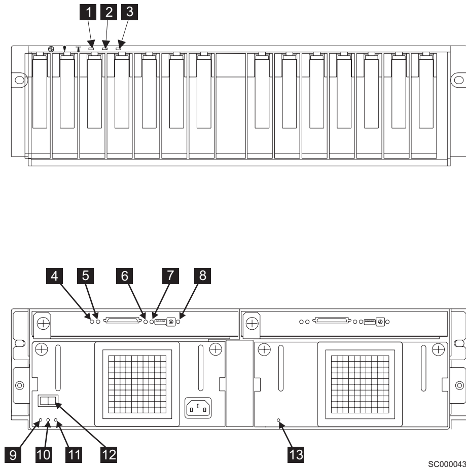
Figure 22. Lights and switches on the 2104 Model DS4
