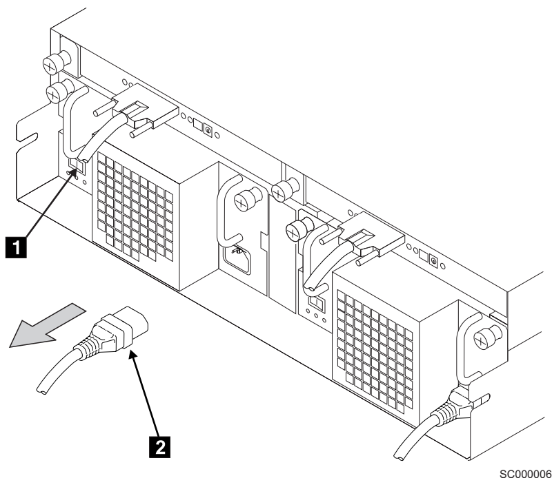
Figure 57. Switching off and disconnecting a fan-and-power-supply assembly
