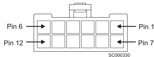
Figure 38. Ground Pins (2104 Model DS4: -48 V)
