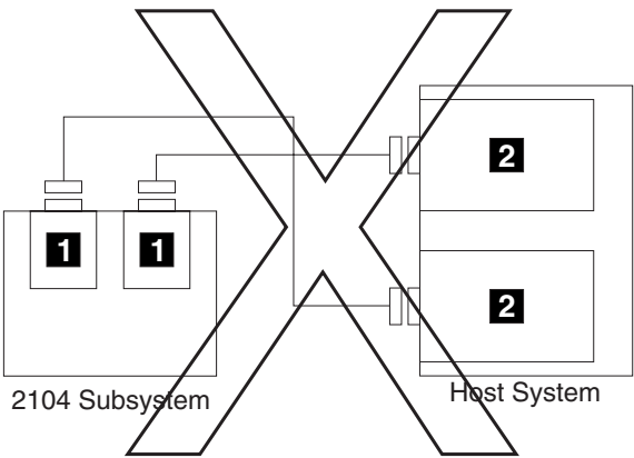
Figure 94. Two adapters in one host system connected to one 2104 Model DS4 or Model TS4 (single-bus mode). This configuration is invalid.
