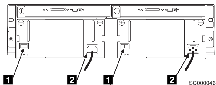
Figure 44. Removing the power from a 2104 Model DS4
