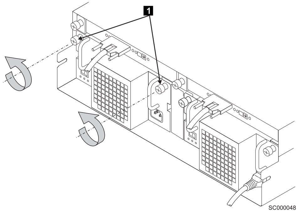
Figure 58. Unscrewing the thumbscrews
