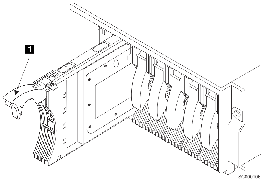
Figure 51. Installing a disk drive module in a 2104 Model DS4
