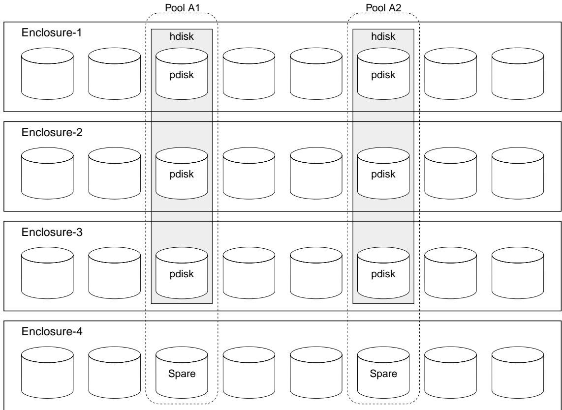
Figure 19. Pools and Hdisk across Enclosures
