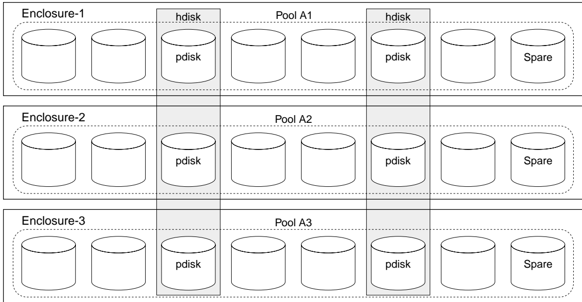
Figure 20. Pools along, and Hdisks across, Enclosures
