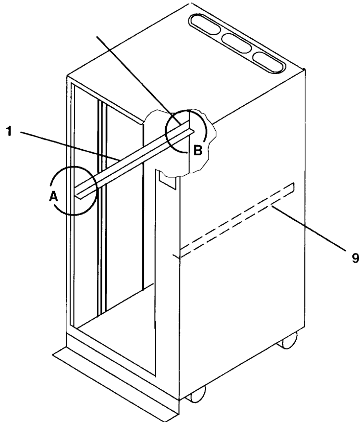
Mounting Hardware For CPU Enclosure
