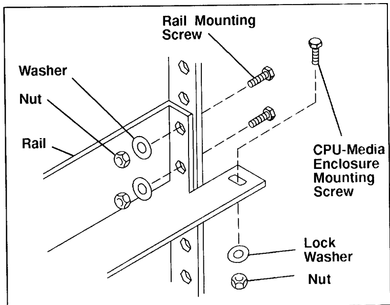
Detail B – Rear of Rail
