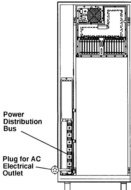
Rear View of Rack
