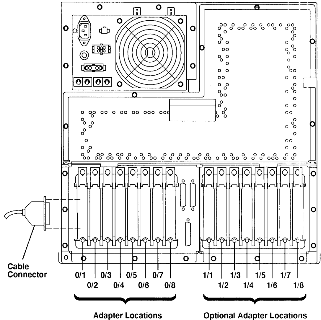
Rear View of CPU-Media Enclosure
