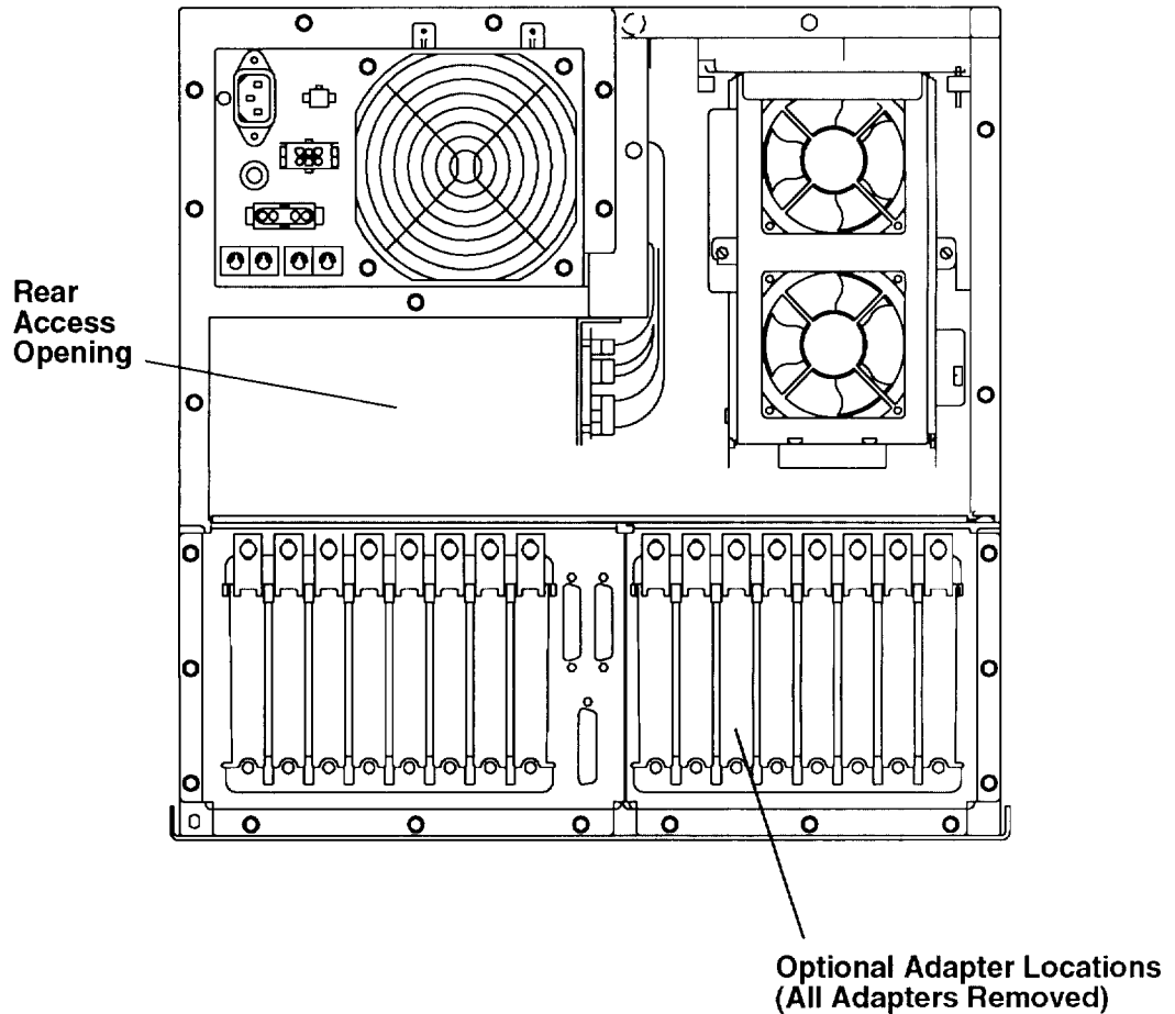
Rear View of CPU-Media Enclosure
