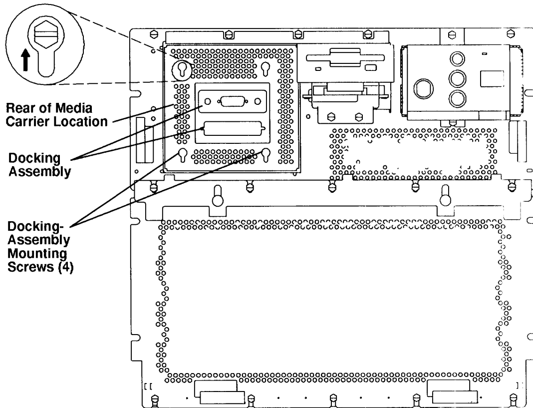
Front View of CPU-Media Enclosure
