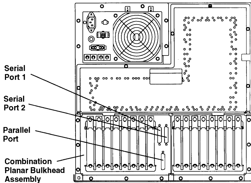
Rear View of CPU-Media Enclosure
