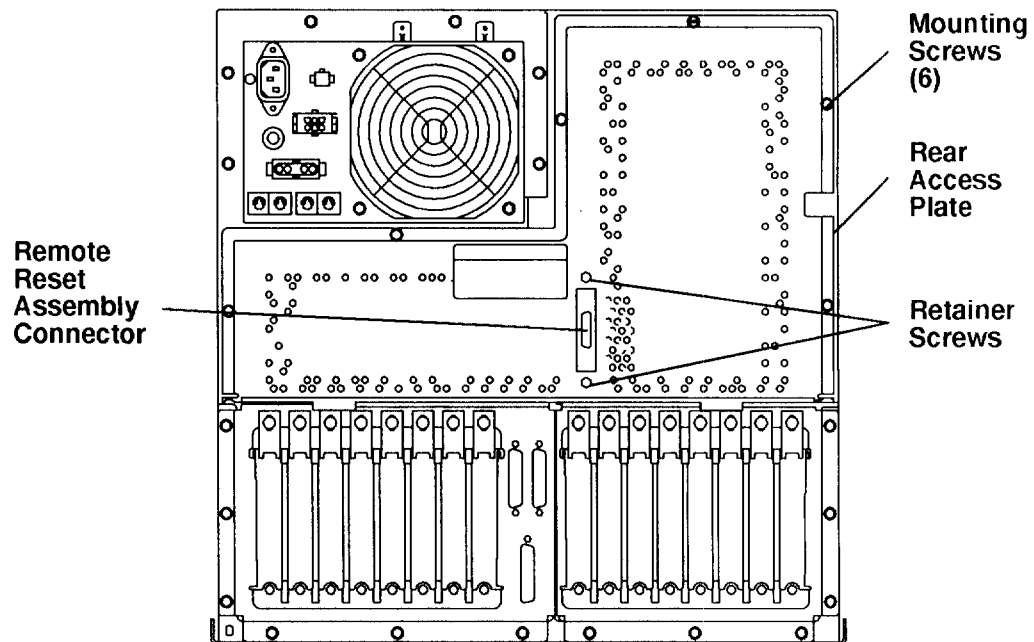
Rear View of CPU-Media Enclosure
