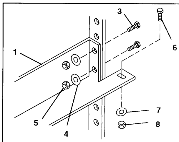
Detail B – Rear of Rail
