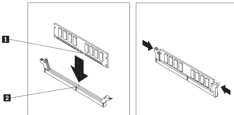
Figura 34. Installing the memory module
