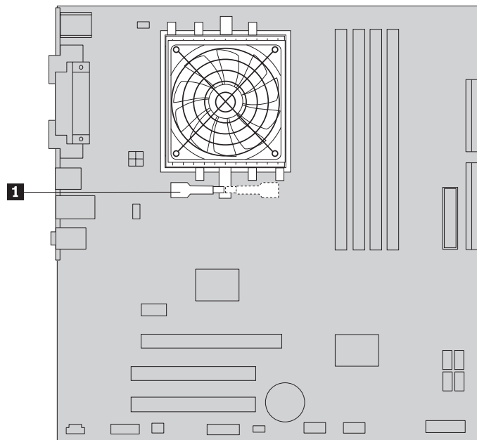
Figura 31. Clamping the heat sink to the plastic retention bracket
