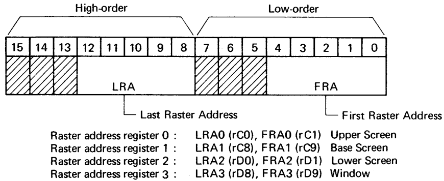
Figure 5.18 Raster Address Register (RAR)
