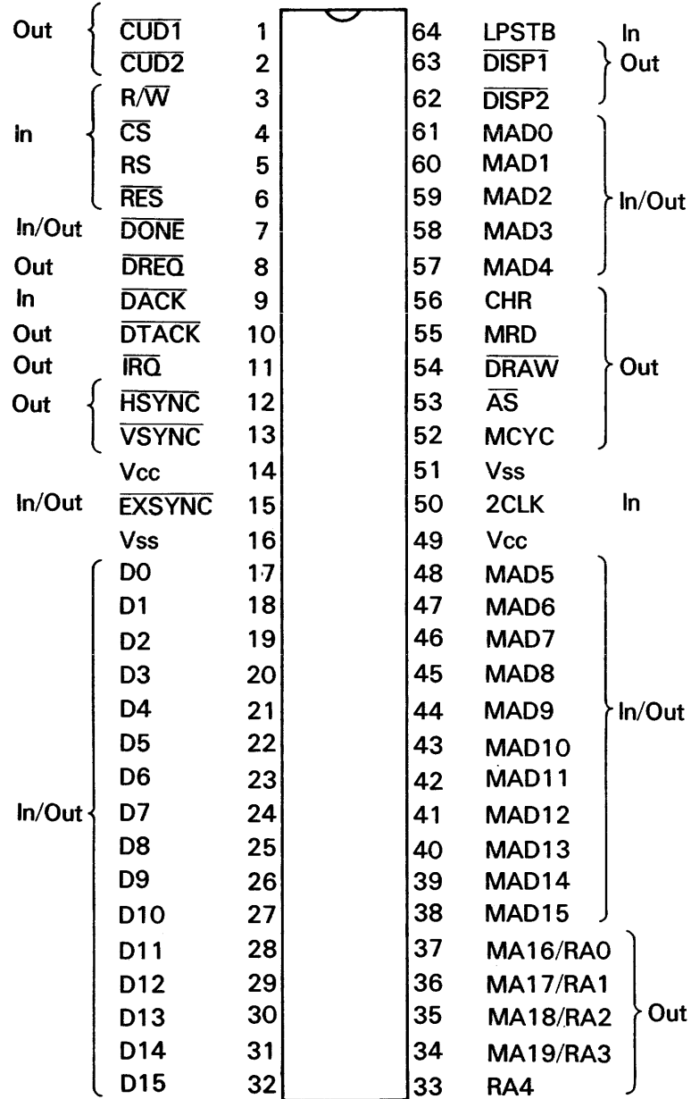
Figure 4.1 Pin Arrangement
