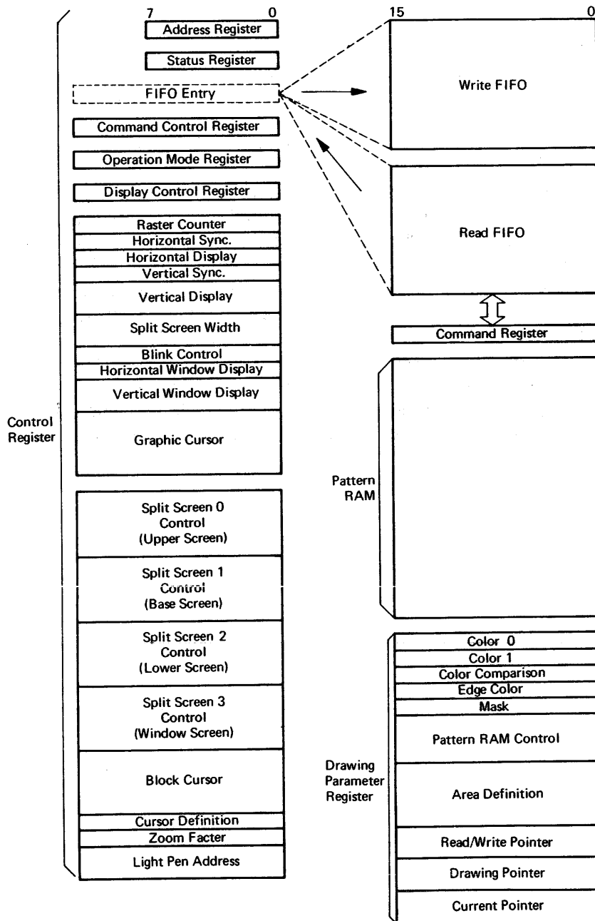
Figure 5.1 Programming Model
