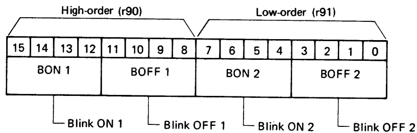
Figure 5.16 Blink Control Register (BCR)
