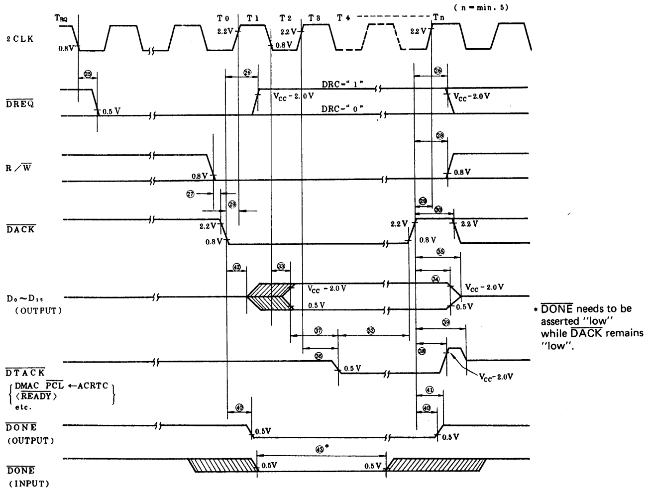
Figure T-4 DMA Read Cycle timing (Memory ← ACRTC)
