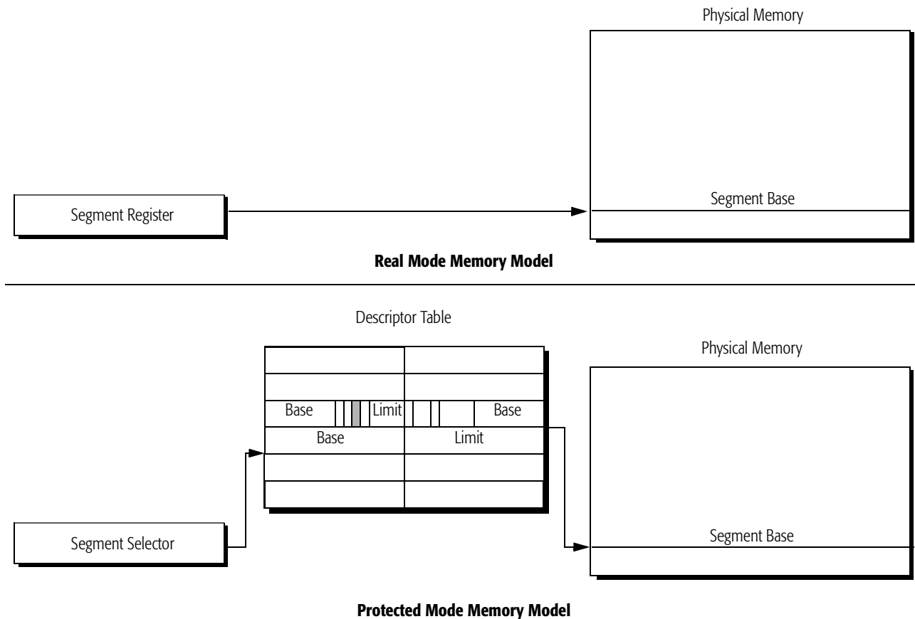
Figure 10. Segment Usage
