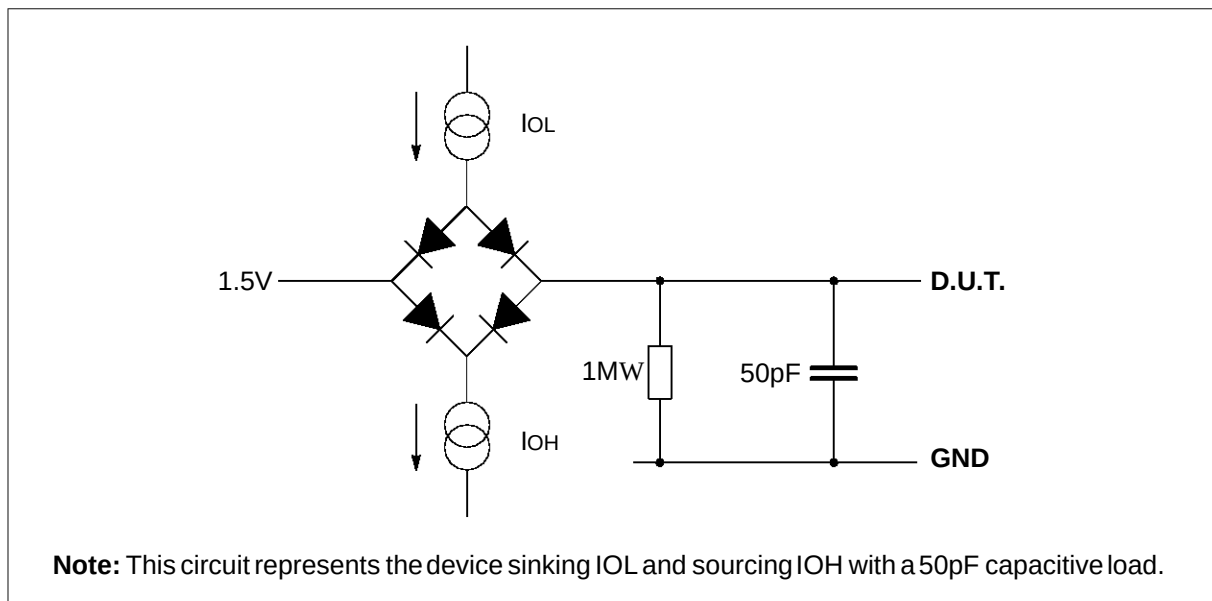
Figure 6.1 Load circuit for AC measurements
