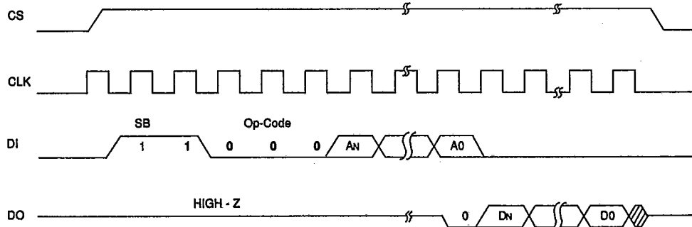
FIGURE 2 - READ MODE
