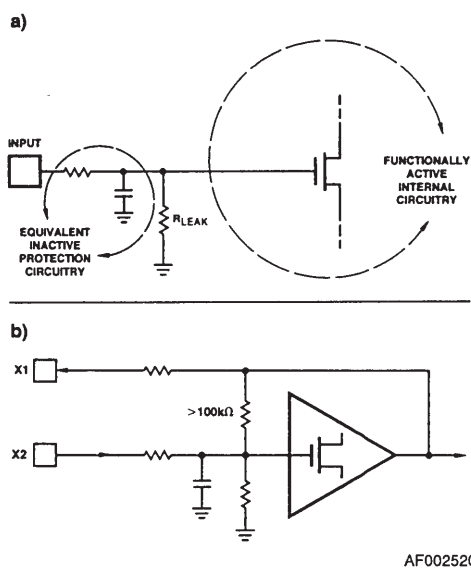
Figure 1-4. Input Circuitry
