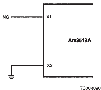
Figure A2. Crystal Input Configuration
