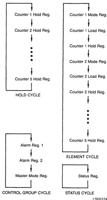
Figure 1-10. Data Pointer Sequencing
