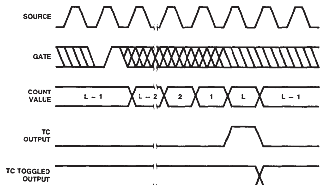
Figure 1-16f. Mode F Waveforms
