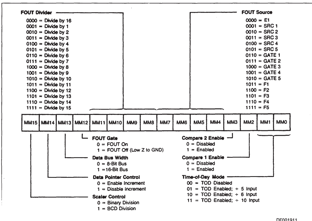
Figure 1-12. Master Mode Register Bit Assignments
