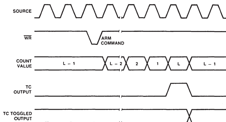
Figure 1-16a. Mode A Waveforms
