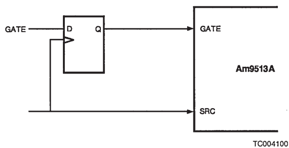
Figure A4. GATE/SRC Configuration Suggestion
