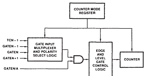
Figure 1-13. Gating Control
