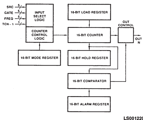
Figure 1-5. Counter Logic Groups 1 and 2
