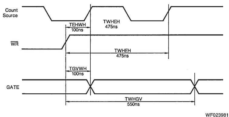
Figure A3. TEHWH/TGVWH Timing Diagram
