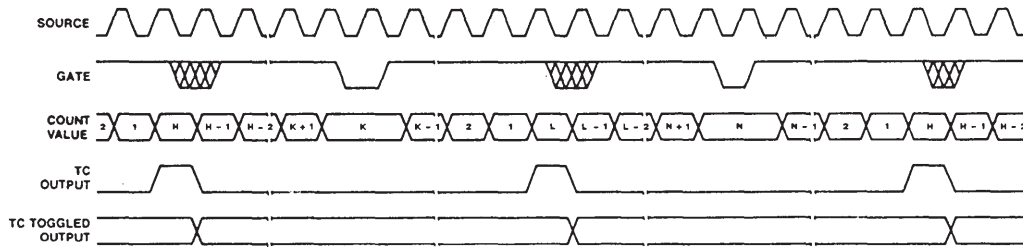
Figure 1-16k. Mode K Waveforms
