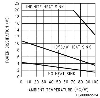
Maximum Power Dissipation (TO-3)
