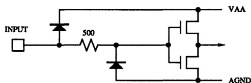
Figure 5. Equivalent Circuit of the Digital Inputs.
