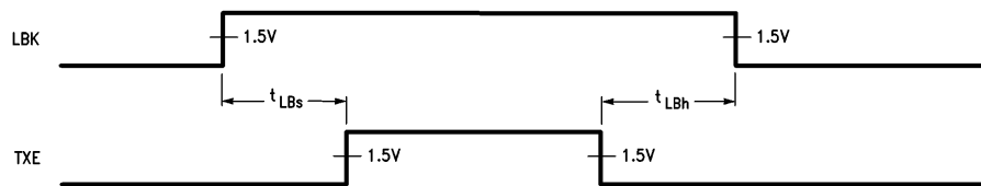
FIGURE 11. Loopback Timing
