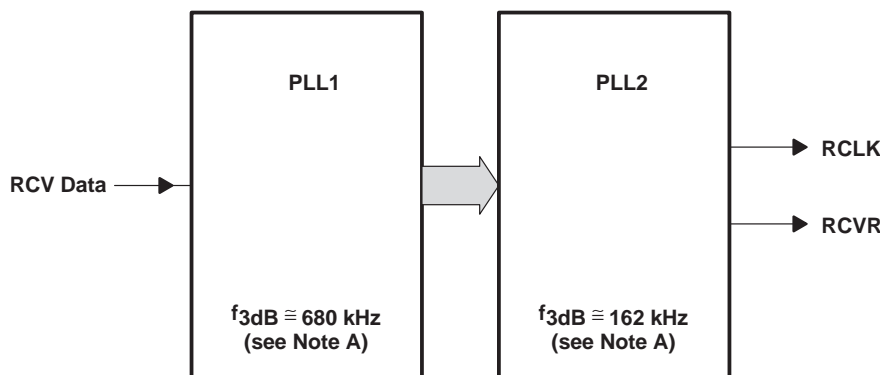
Figure 3. Dual-PLL Arrangement
