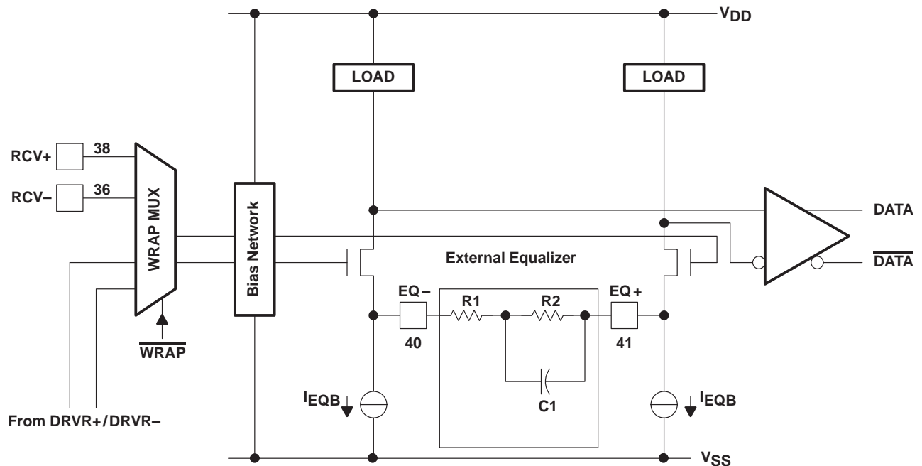
Figure 2. Line Receiver/Equalizer
