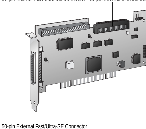
50-pin Internal Fast/Ultra-SE Connector 68-pin Internal LVD/SE Connector
