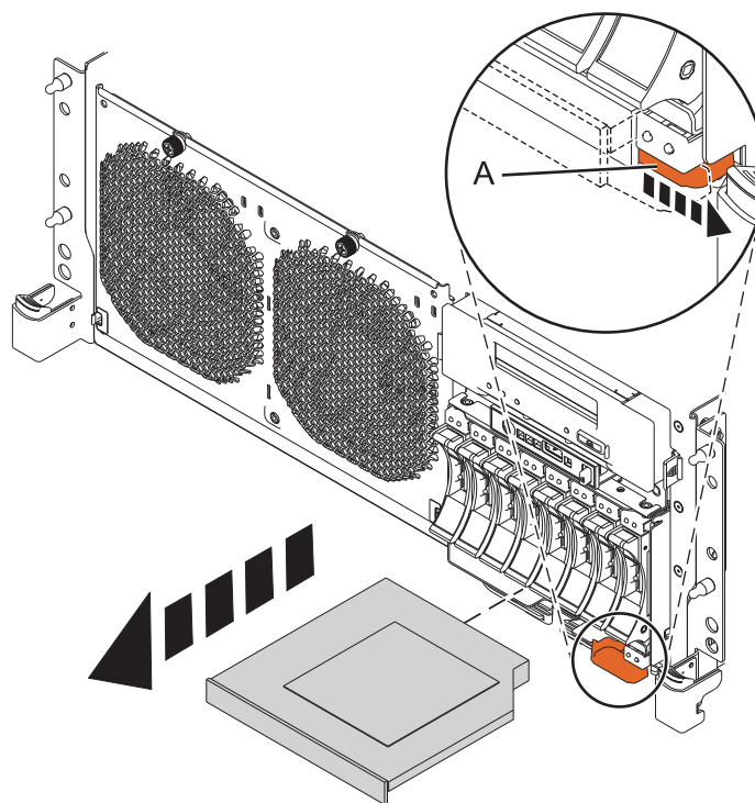
Figure 4. Removal of a Slimline media device
