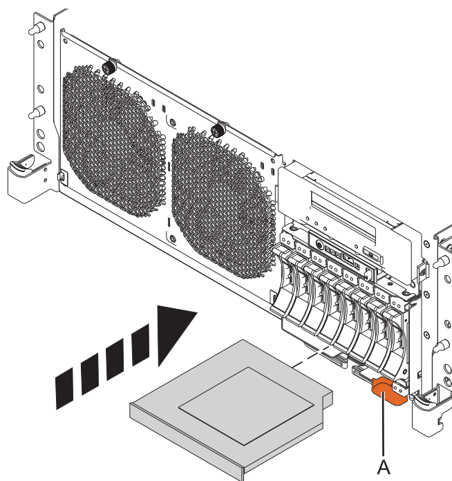
Figure 15. Installation of a Slimline media device
