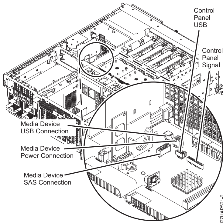
Figure 21. Media device connections
