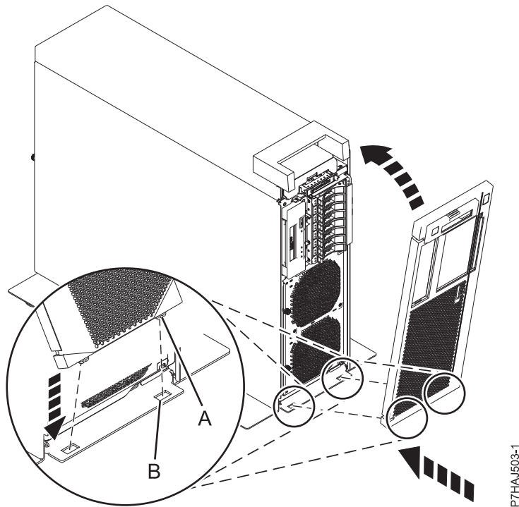
Figure 30. Installing the front cover
