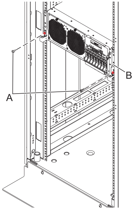
Figure 38. Placing the system in the service position
