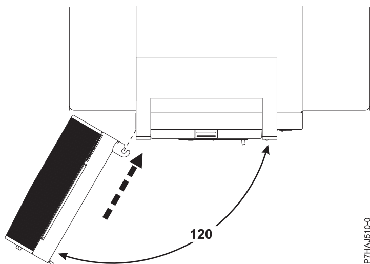
Figure 31. Installing the front door
