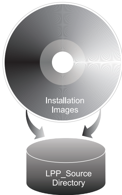
Figure 4. An example of an LPP_Source resource.. This illustration shows that when an LPP_Source resource is created, installation images are copied from the product CD-ROM to the LPP_Source directory.
