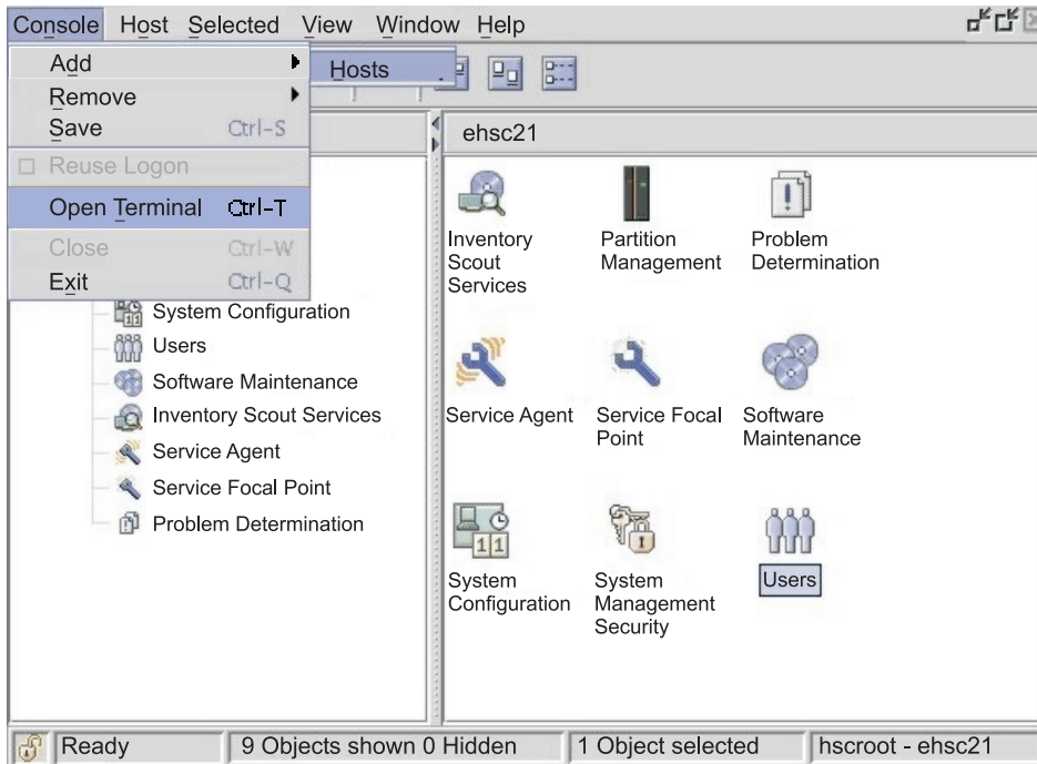
Figure 6. Adding a host using the console menu.. This illustration shows how to navigate from the console menu to the hosts selection. To add the partition as a host in the HMC interface, select Console from the menu bar, then select Add , and then select Hosts .
