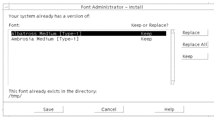
FIGURE 3-3 Conflict Dialog
